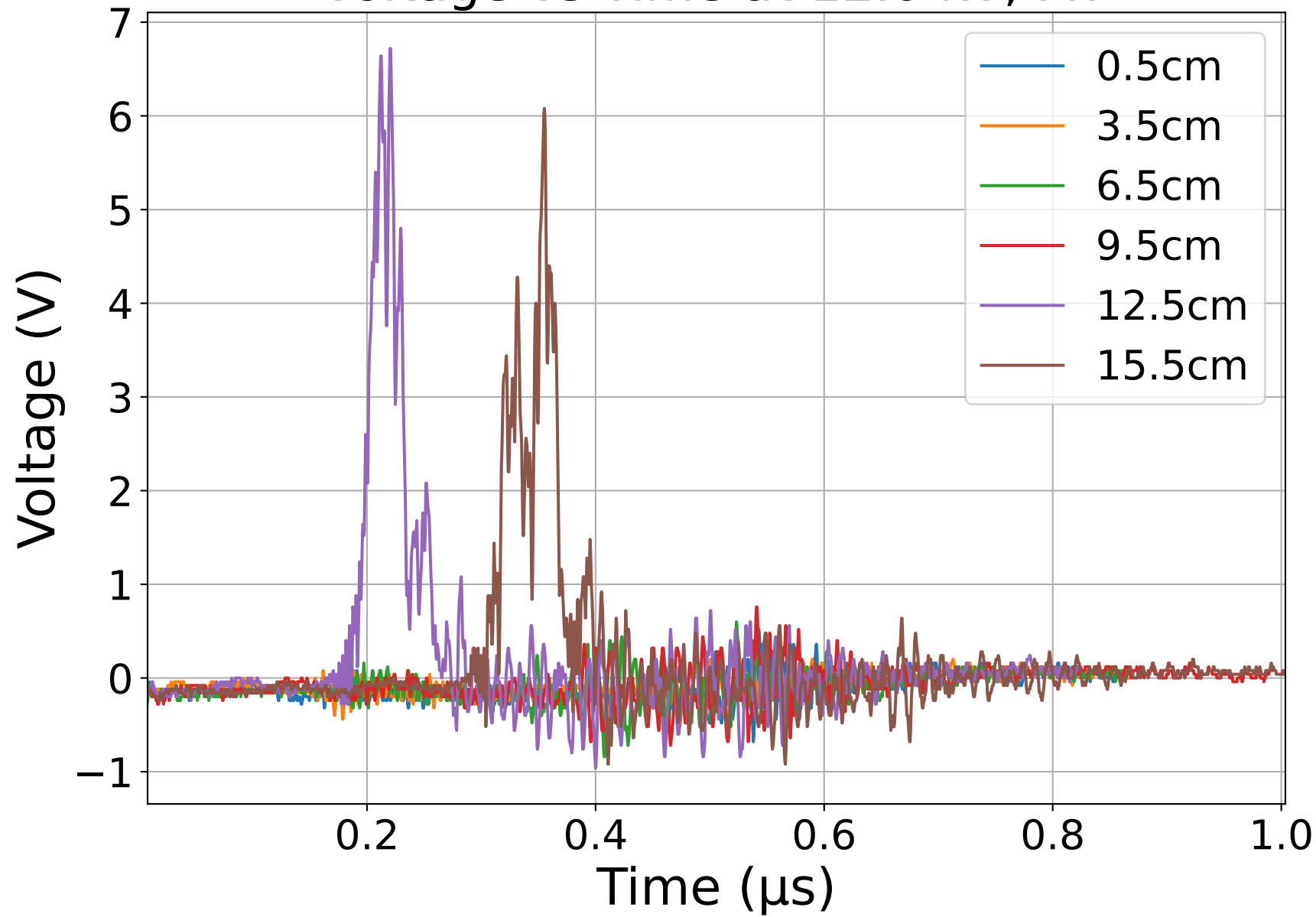
Voltage vs Time at 12.0 kV, M7
