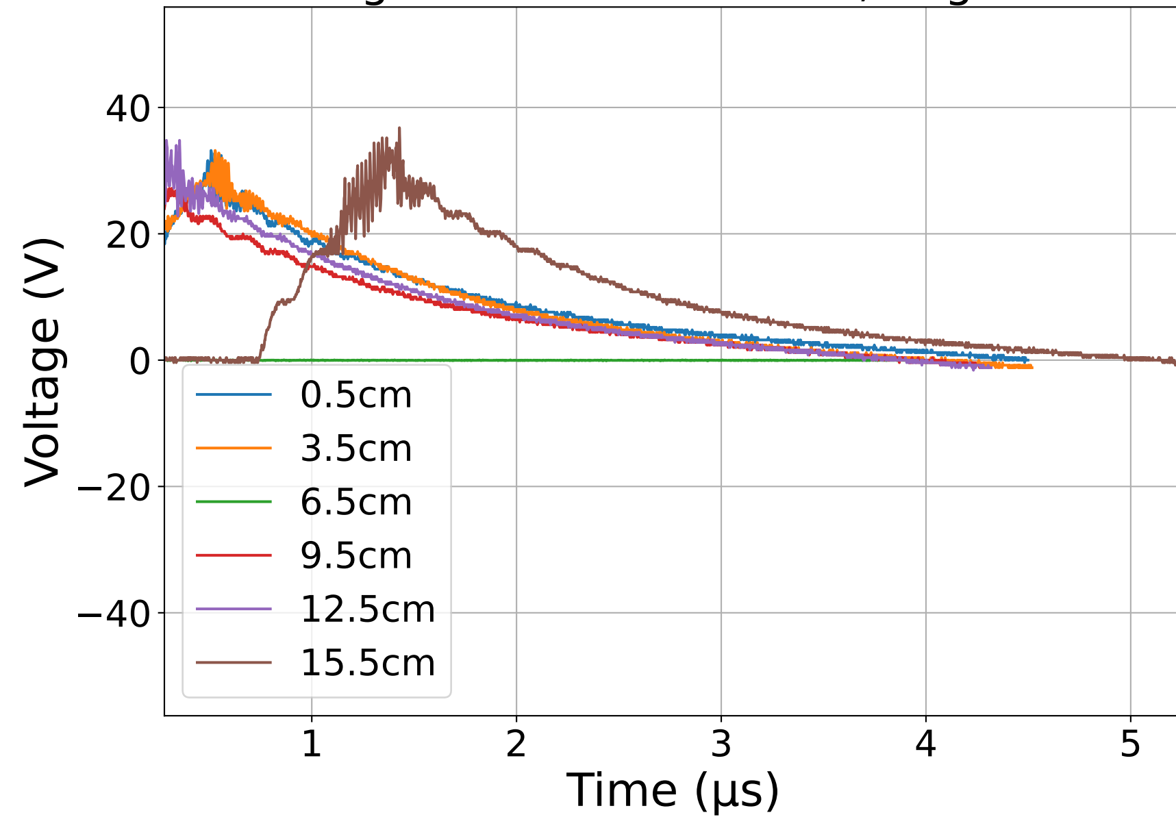
Voltage vs Time at 12.0 kV, Rogowski
