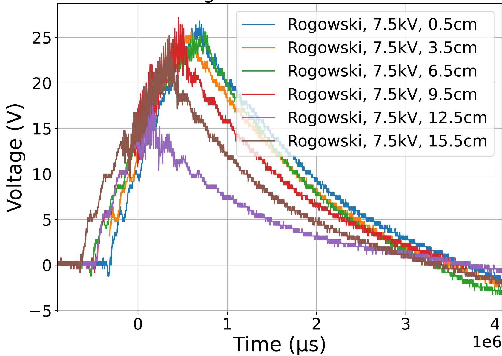
Voltage vs Time at 7.5 kV
