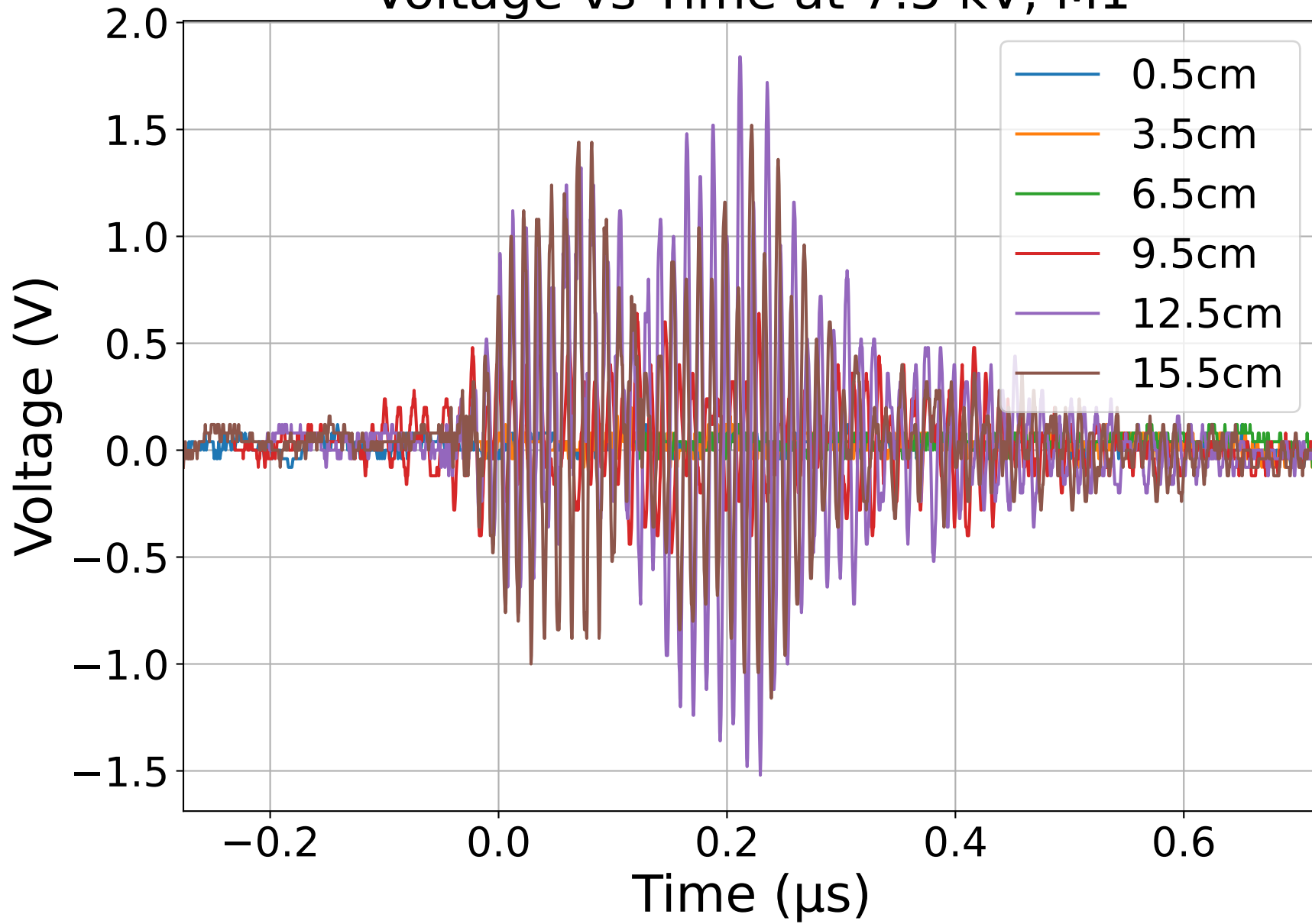
Voltage vs Time at 7.5 kV, M1
