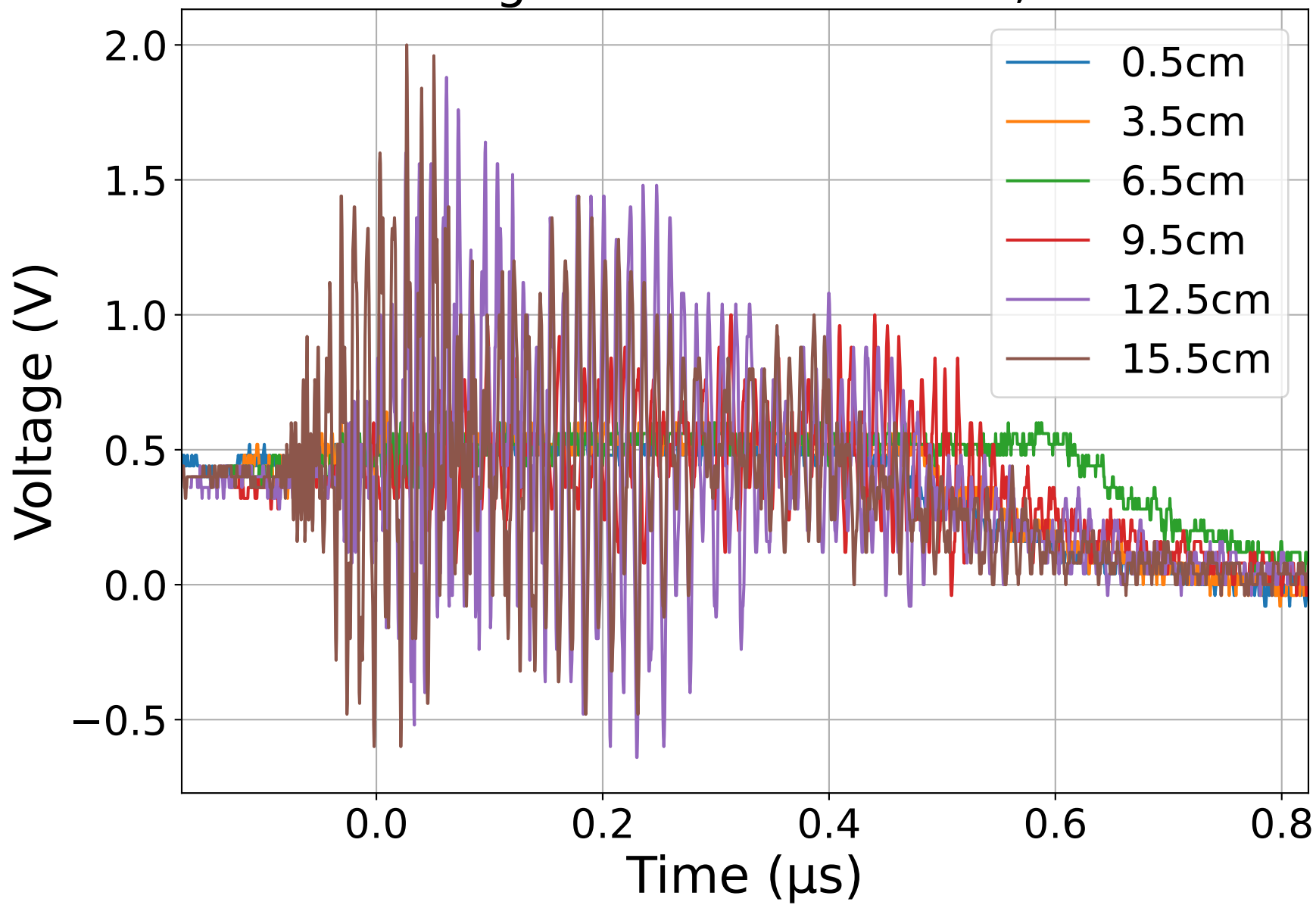
Voltage vs Time at 7.5 kV, M4
