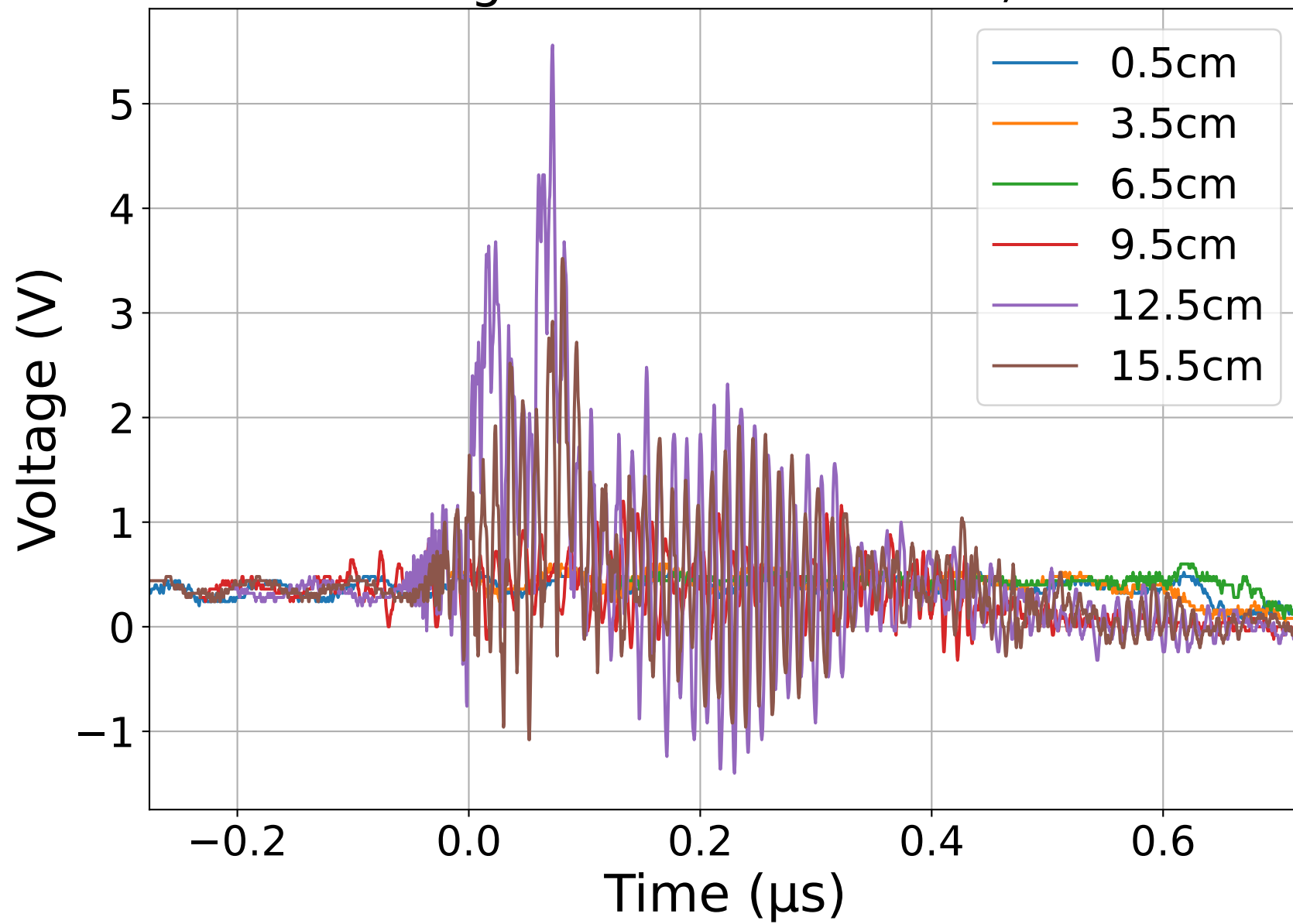
Voltage vs Time at 7.5 kV, M5
