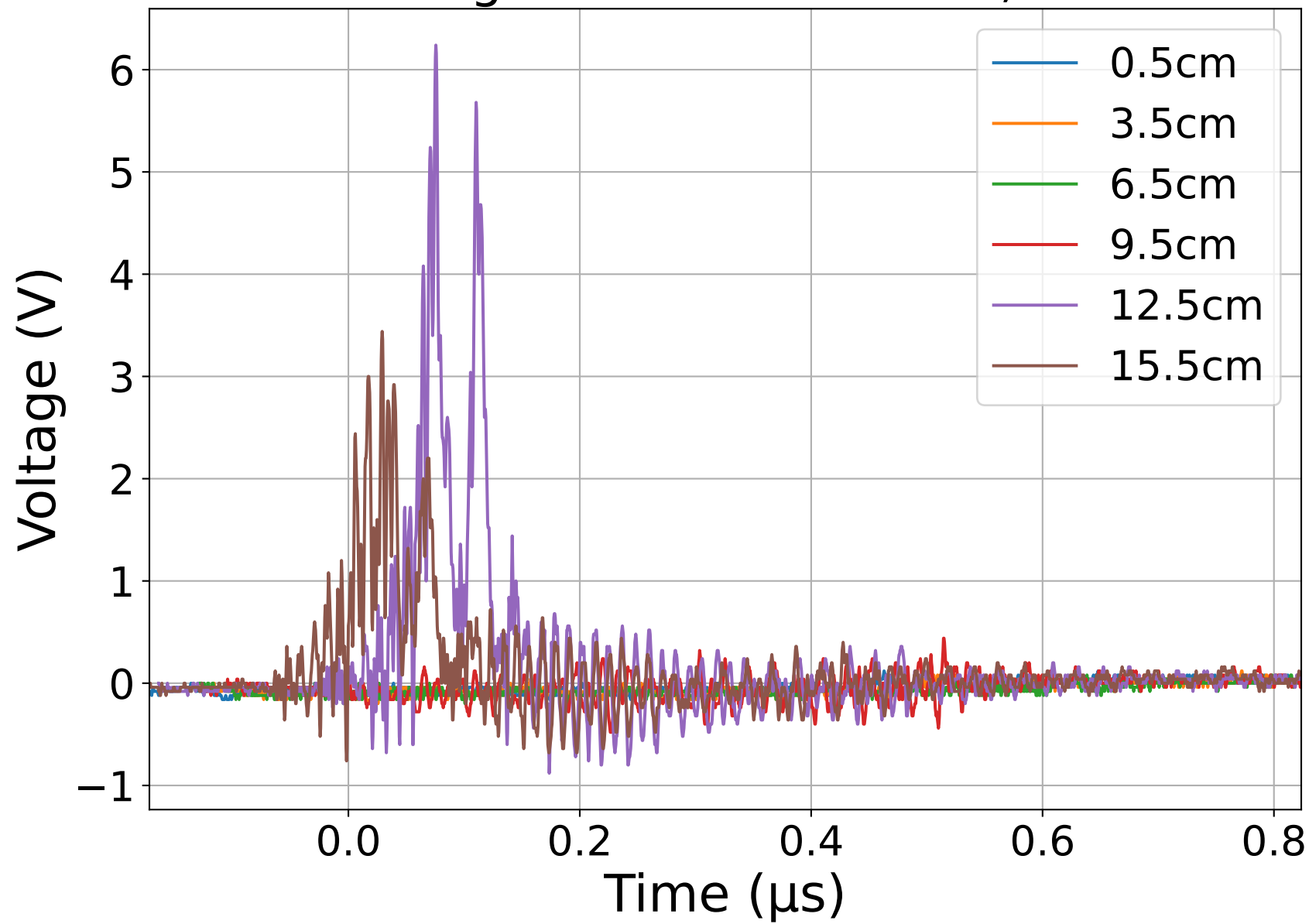
Voltage vs Time at 7.5 kV, M7
