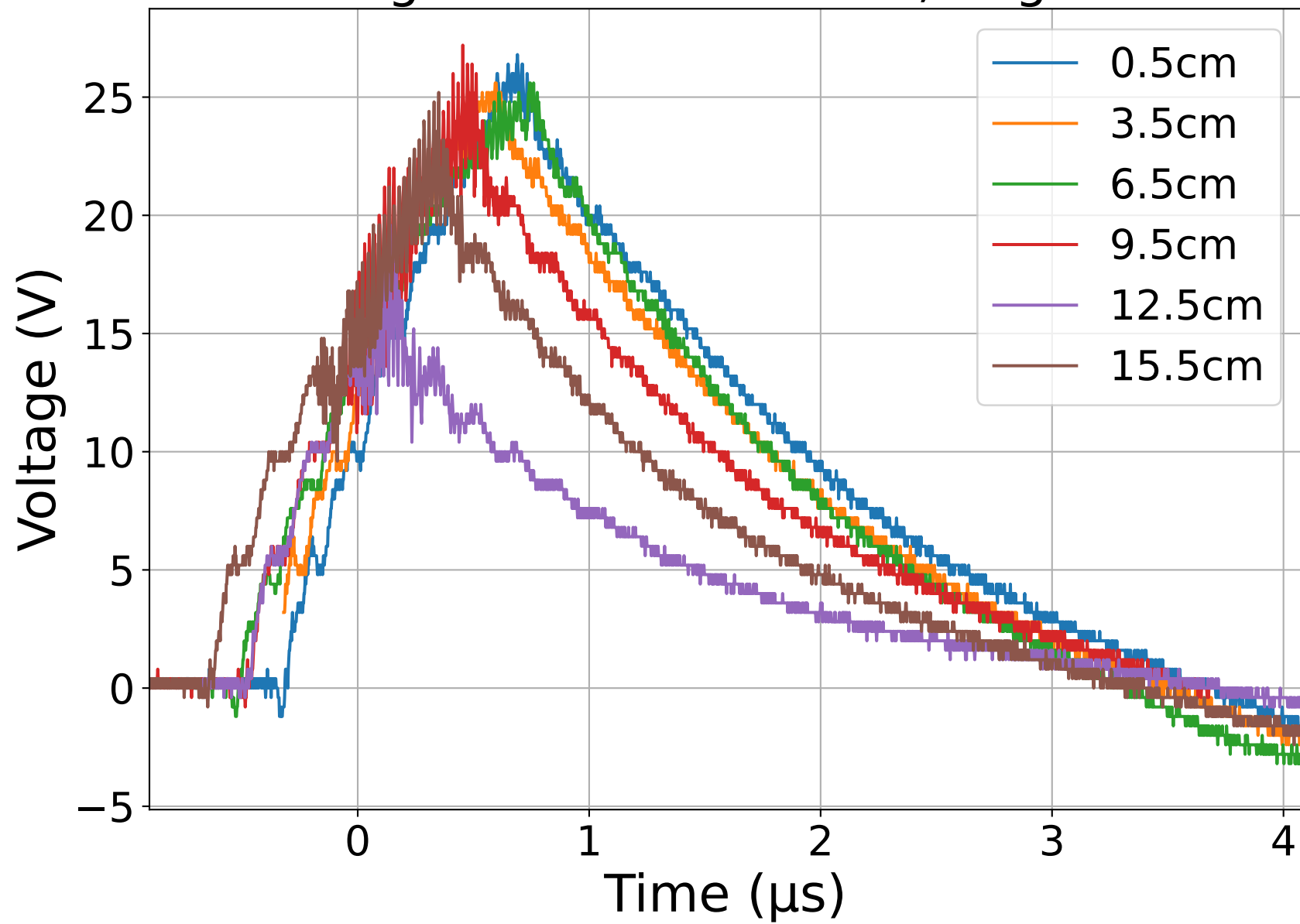
Voltage vs Time at 7.5 kV, Rogowski
