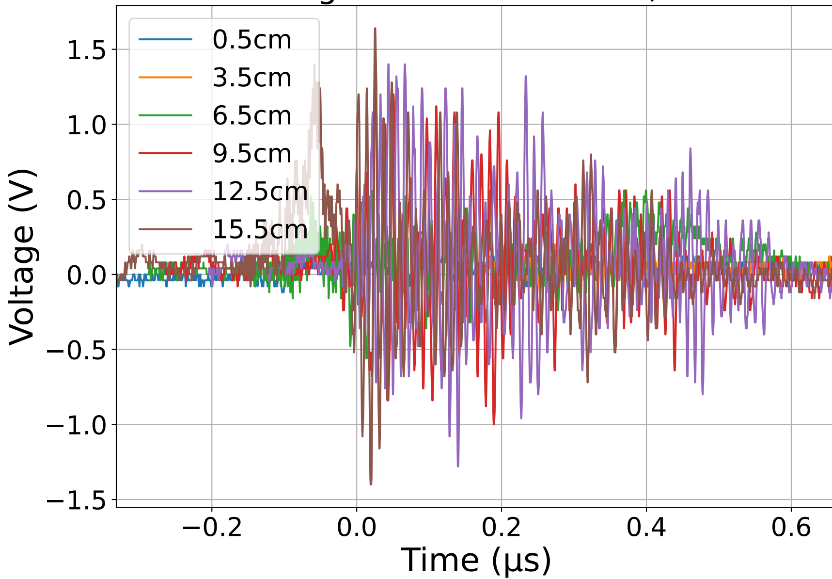
Voltage vs Time at 9.0 kV, M1
