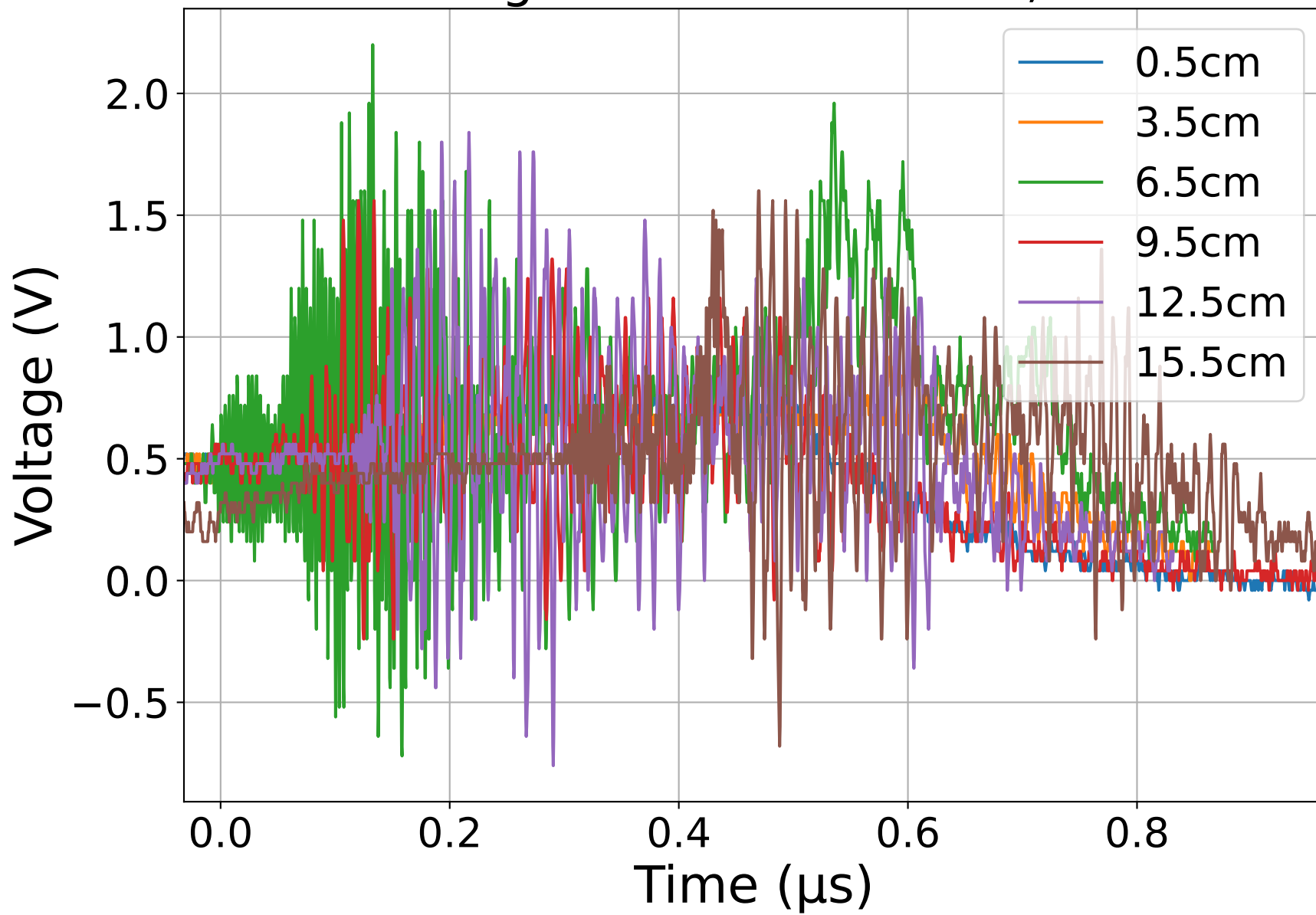
Voltage vs Time at 9.0 kV, M4
