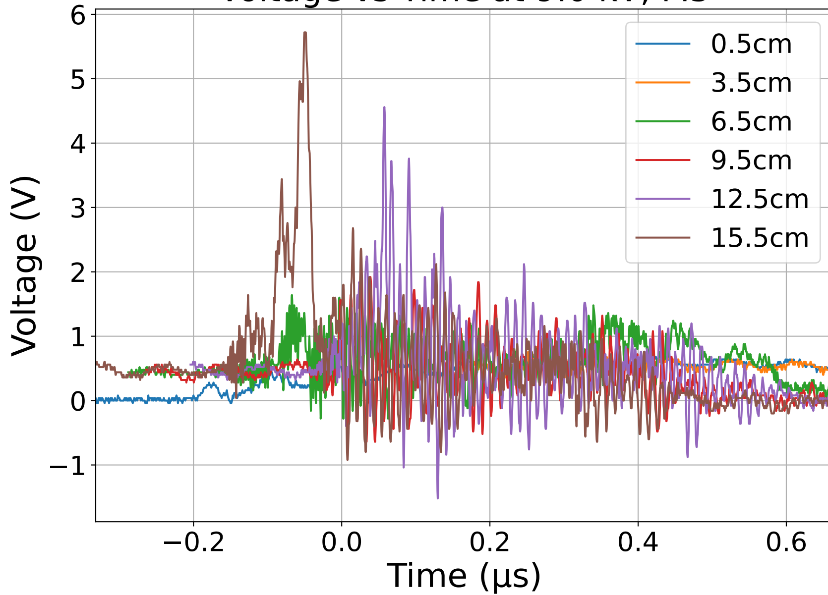
Voltage vs Time at 9.0 kV, M5
