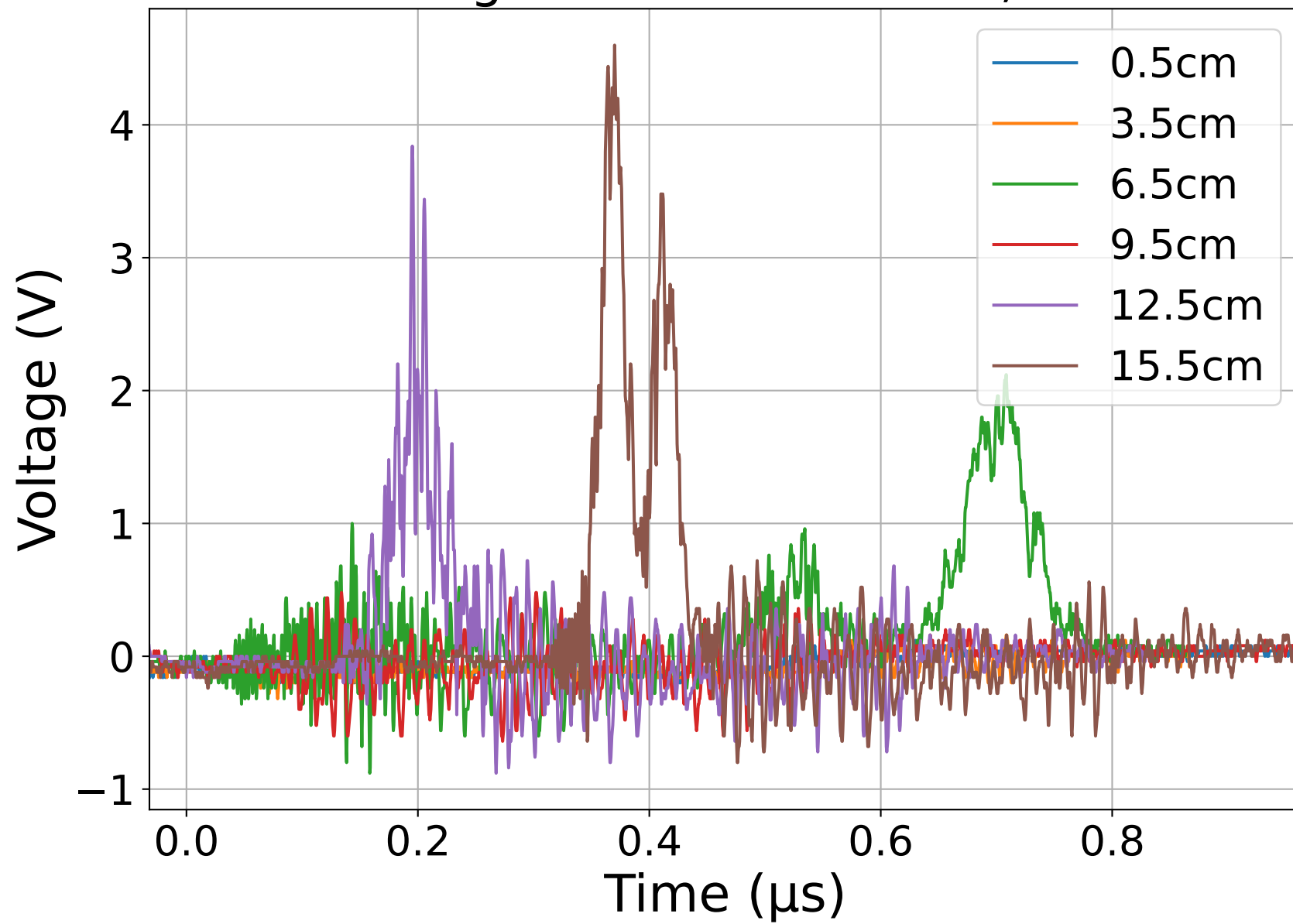
Voltage vs Time at 9.0 kV, M7
