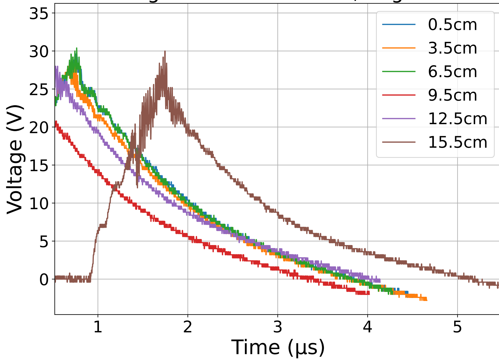
Voltage vs Time at 9.0 kV, Rogowski
