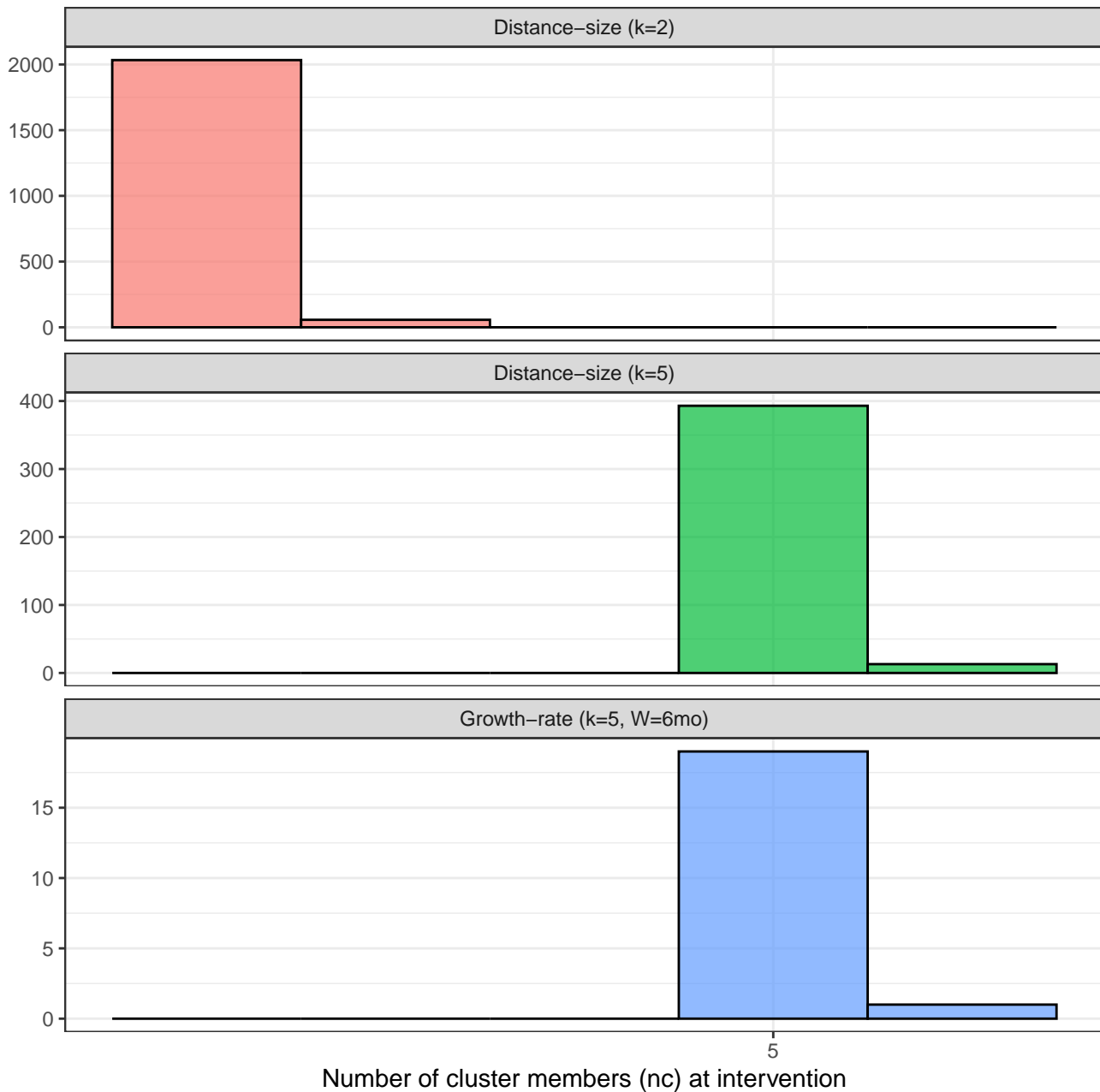
Distribution of Cluster Sizes at Intervention Time
