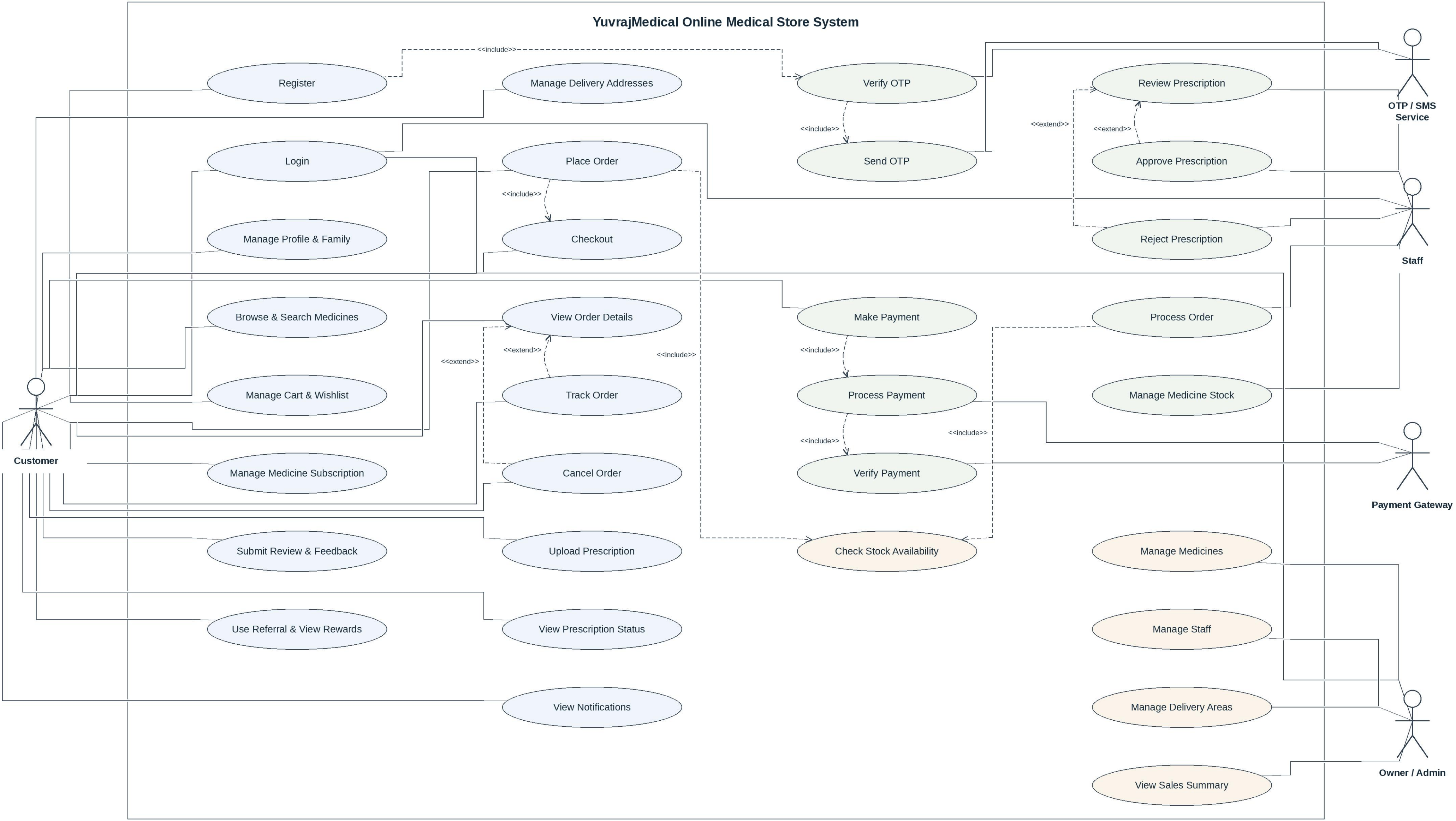
UML Use Case Diagram — Intermediate Detail
