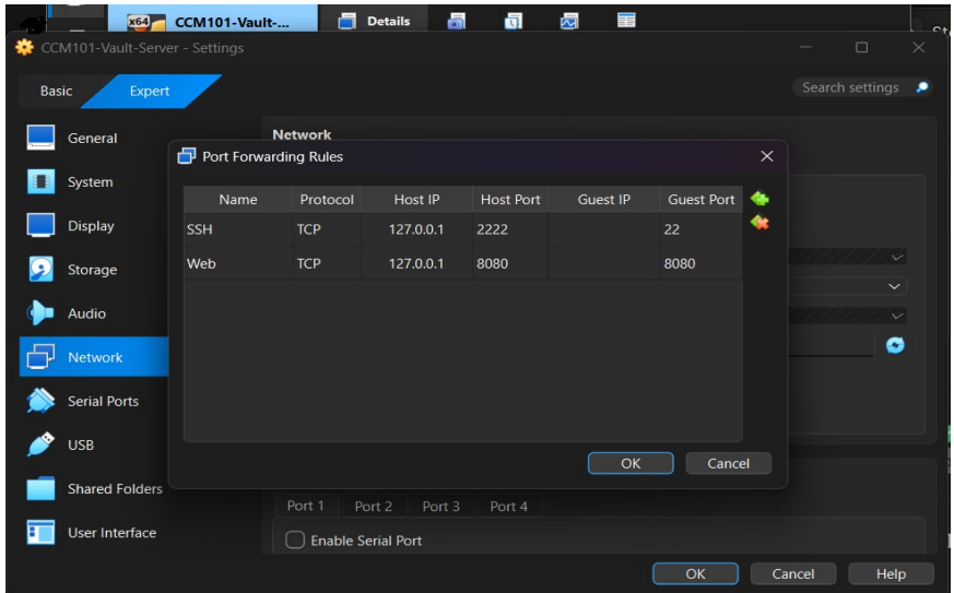
Figure 2. VirtualBox Port Forwarding Rules
