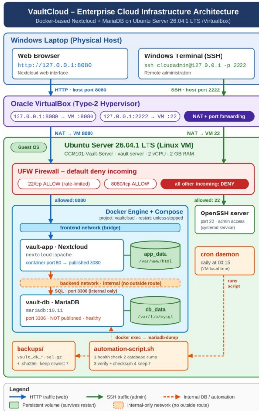
Figure 1. Enterprise Cloud Infrastructure Architecture
