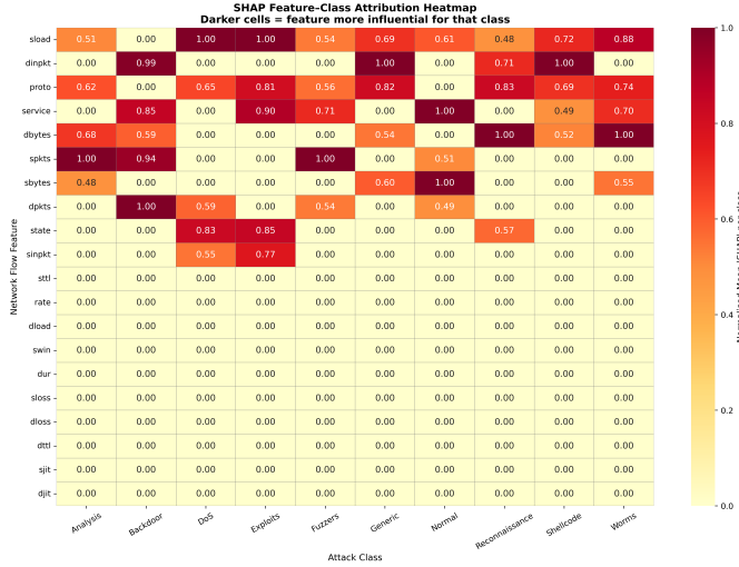
Fig. 3. Global SHAP Explainability Heatmap
