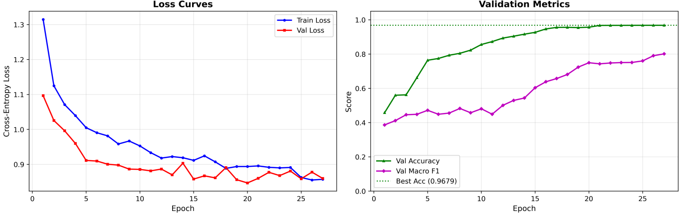
Fig. 2. Training History Of LIDS-T
