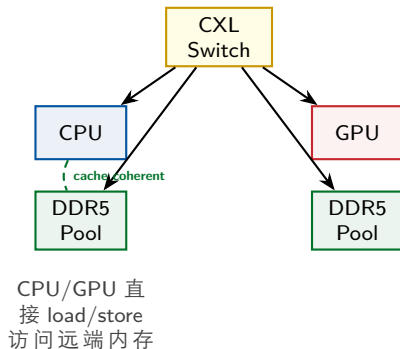
CXL Fabric (Memory Semantic)
