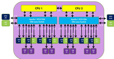
Figure: KM 框图
