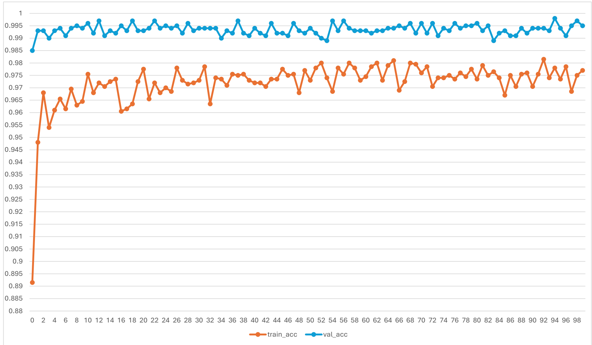
EfficientNetB3 (Phase 2)
