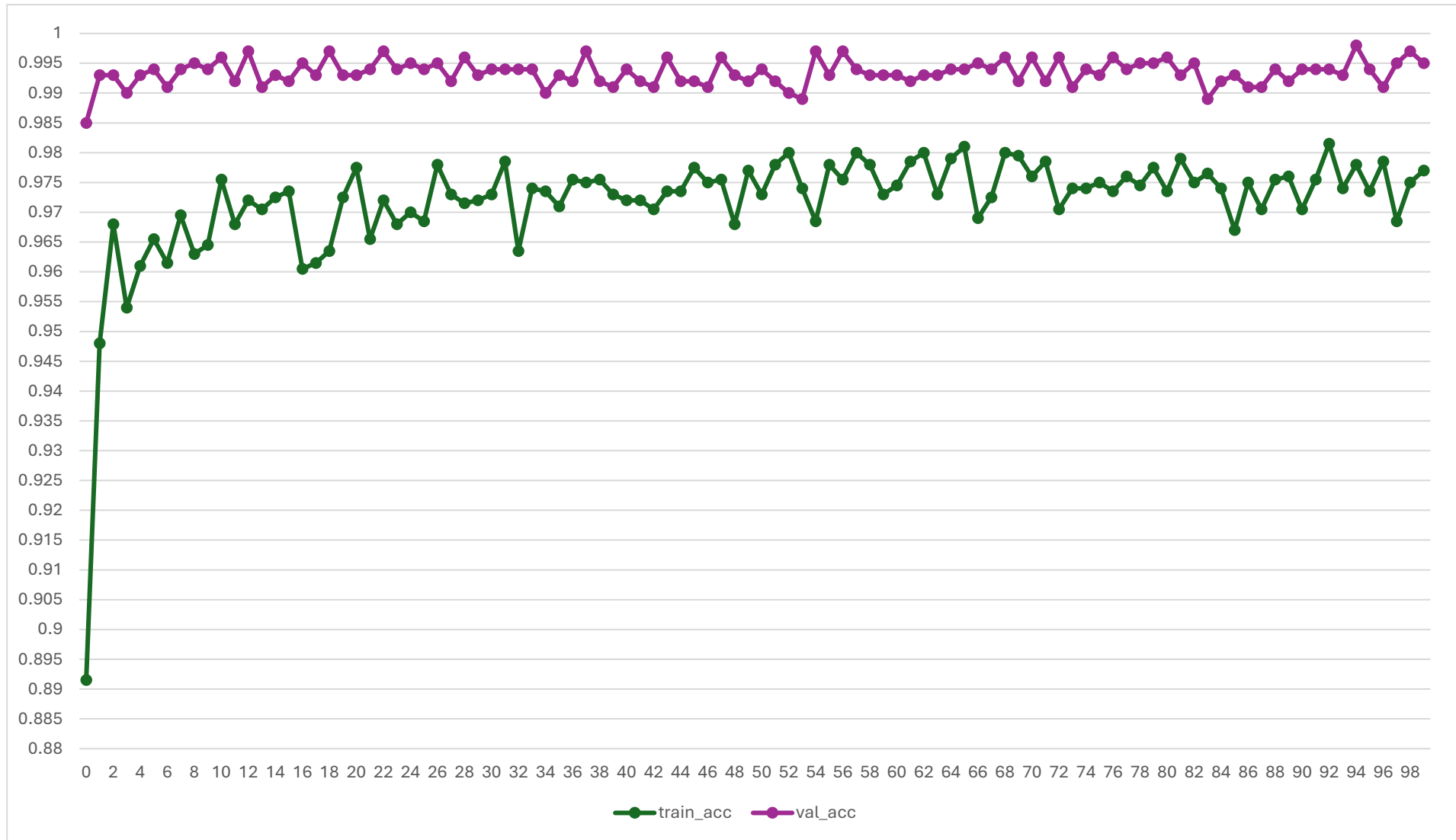
EfficientNetB3 (Phase 1)
