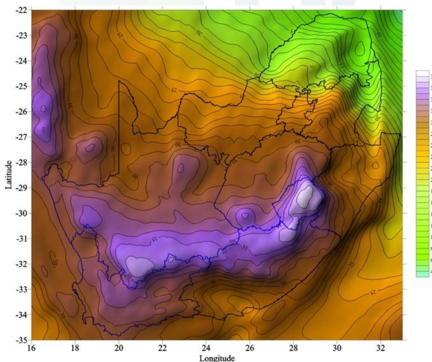
Figure 1. South African Geoid Model 2010
