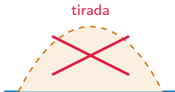
(b) Bouguer
