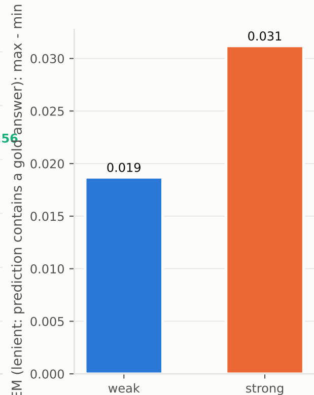
Spread across chunkers
