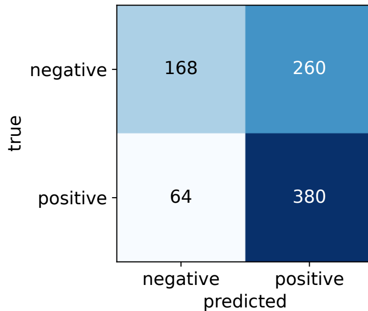
SST-2: TextBlob
