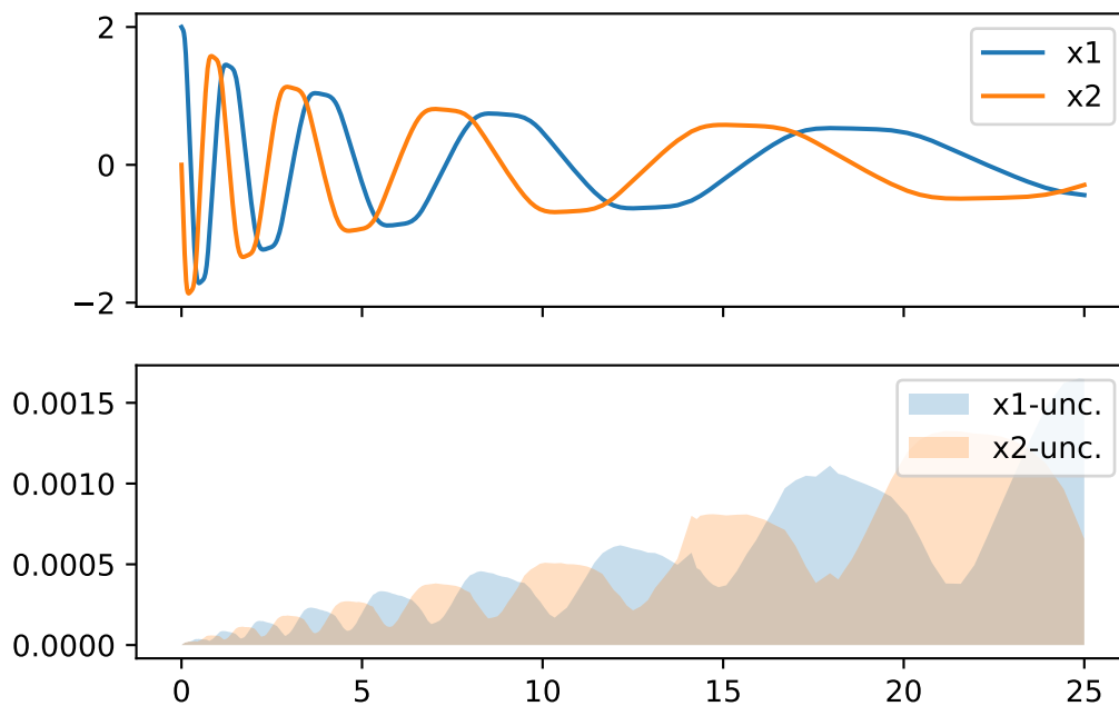
EK0 Solution
