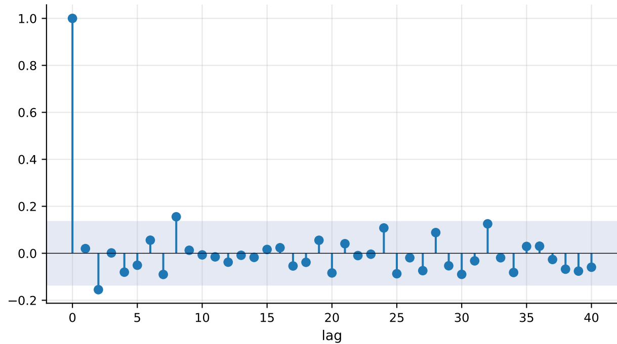
PACF — anchor (longest history)
