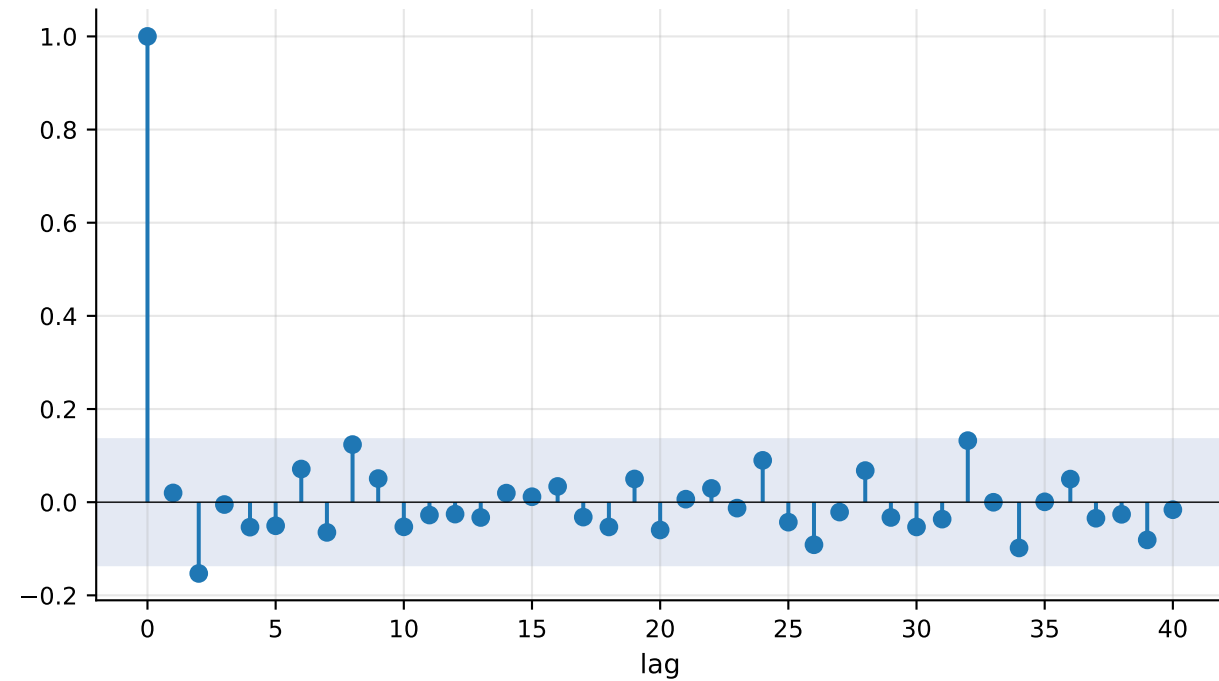
ACF — anchor (longest history)
