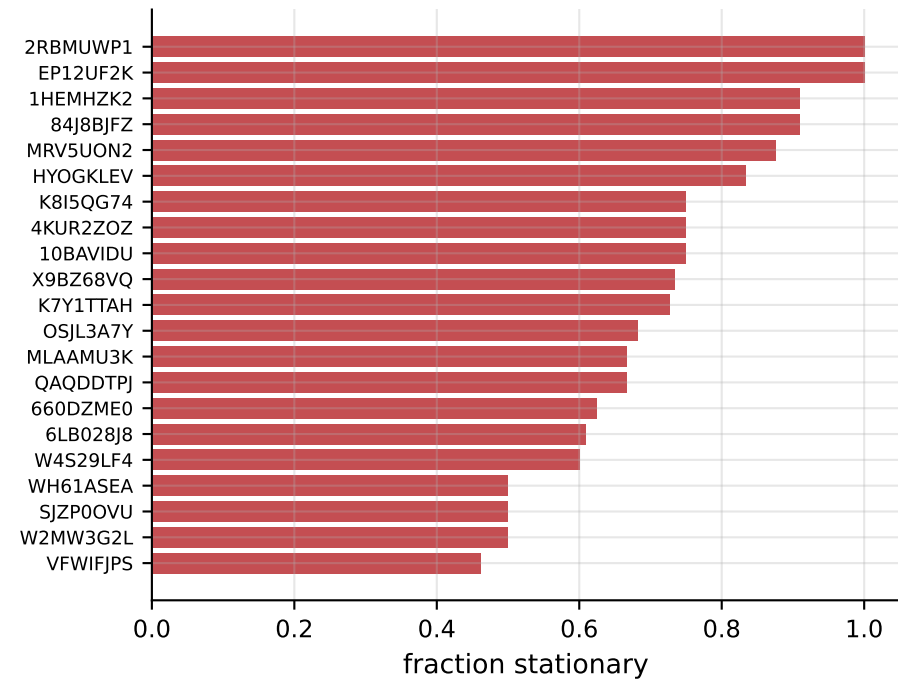
Fraction stationary by code
