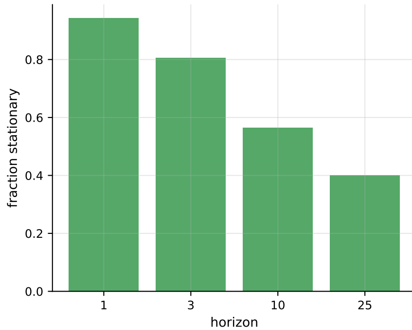
Fraction stationary by horizon
