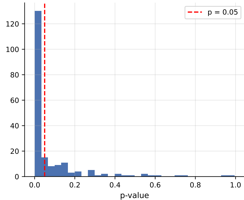
ADF p-value distribution
