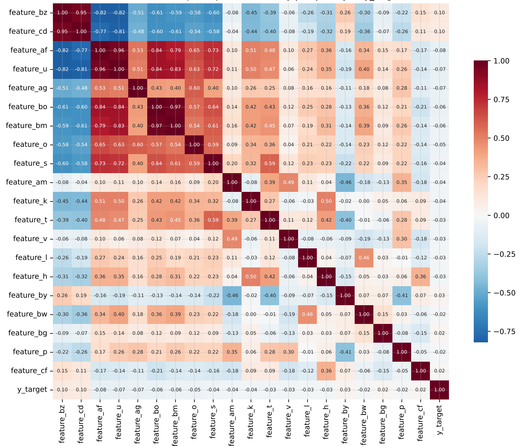
Correlation heatmap — top 20 features (by |corr| with y) + y_target
