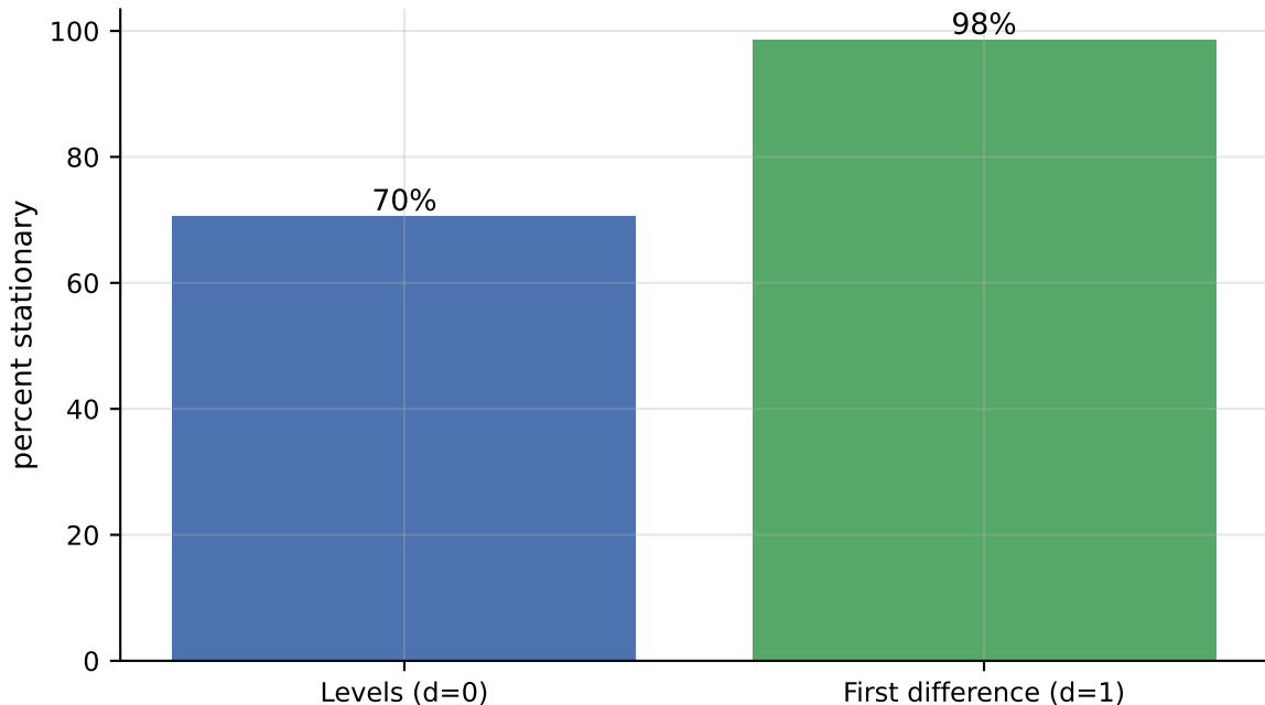
ADF stationary share: before vs after first differencing
