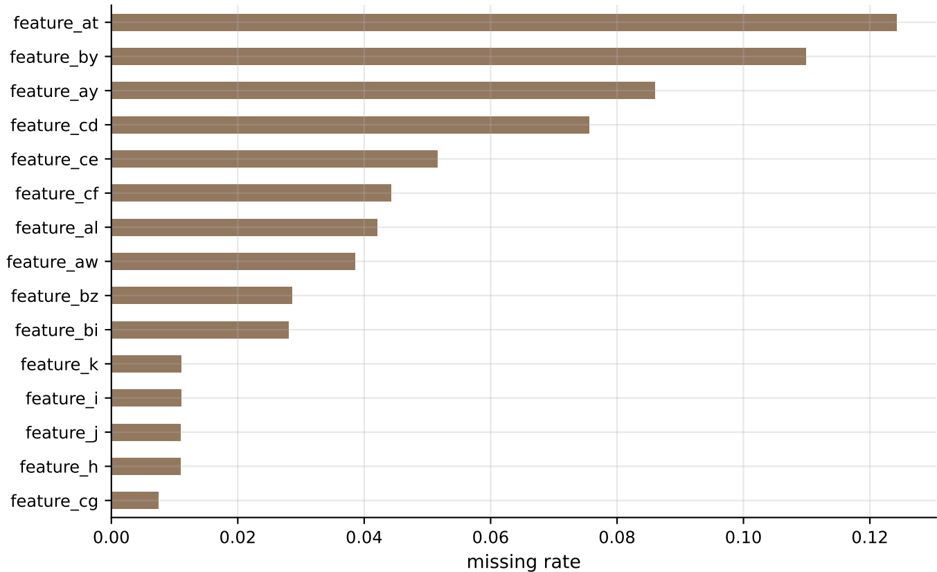
Top 15 features by missingness (500k sample)
