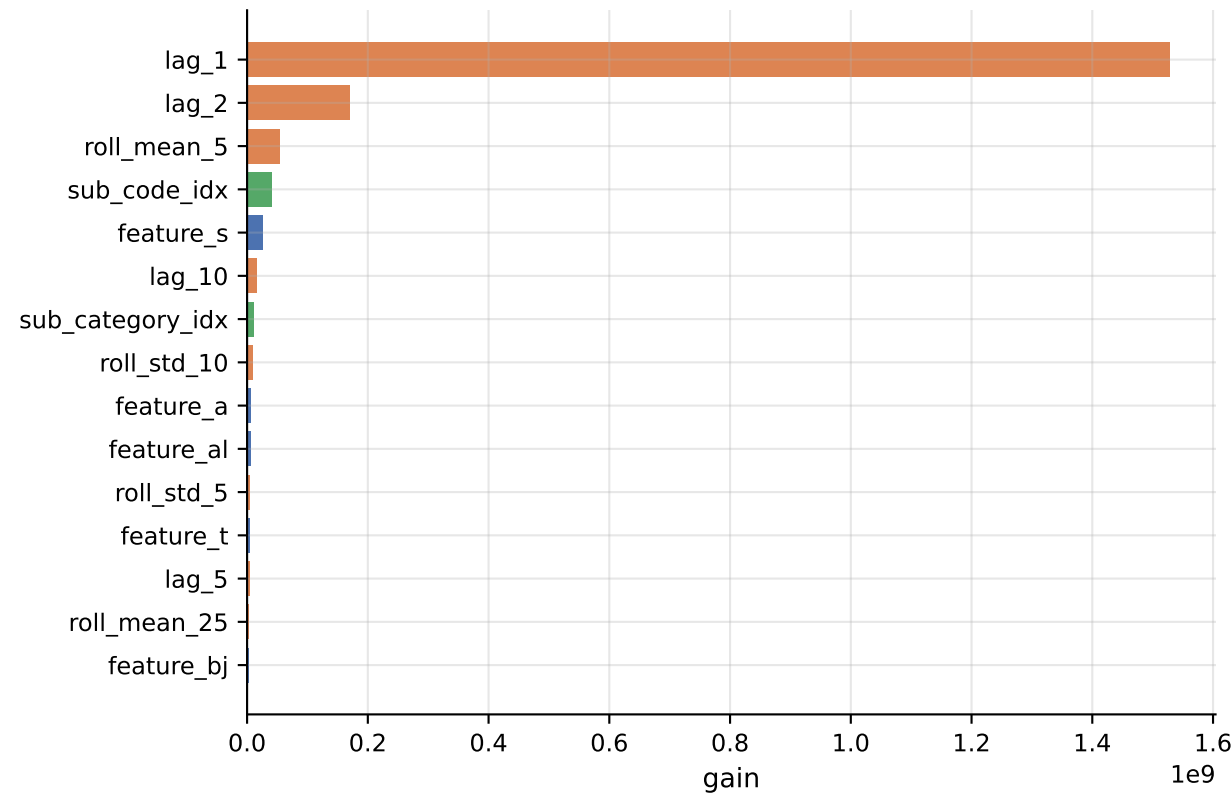
H10 top 15 features by gain
