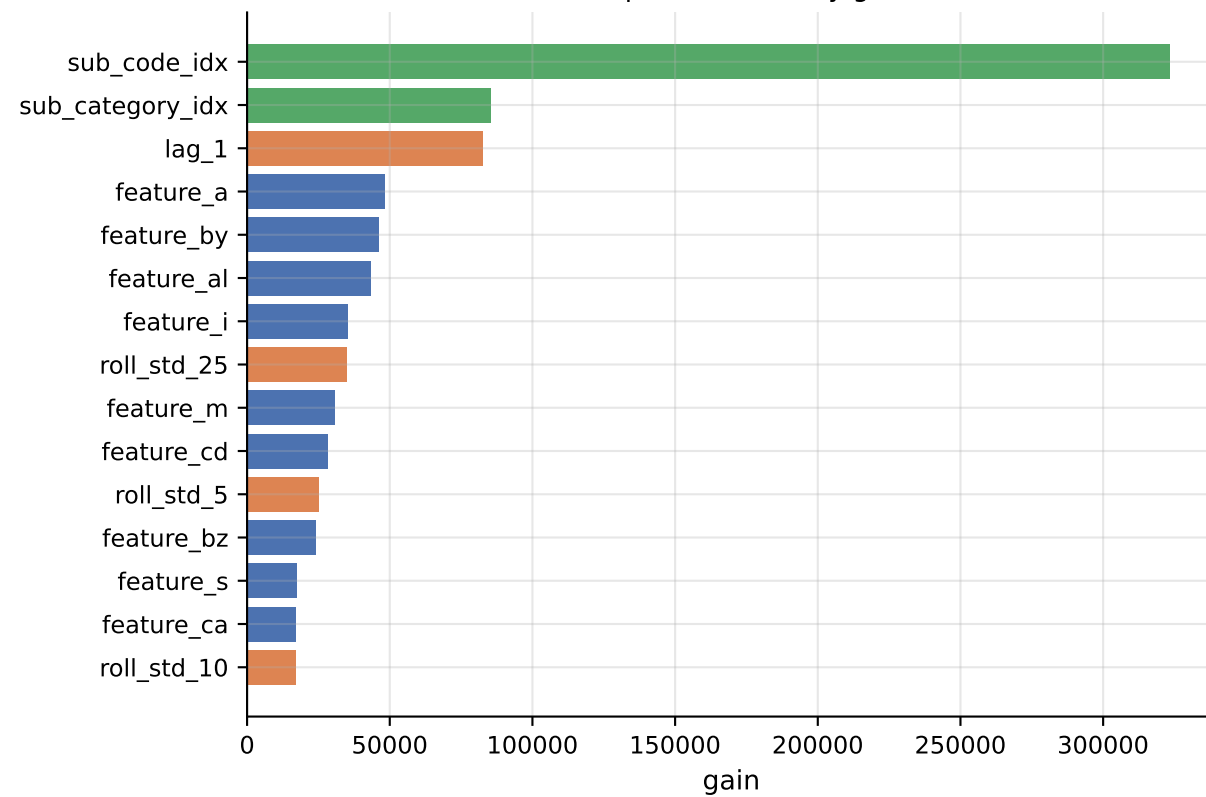
H10 top 15 features by gain
