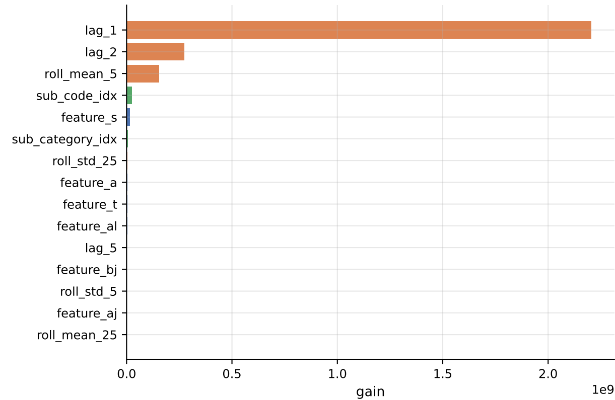
H25 top 15 features by gain
