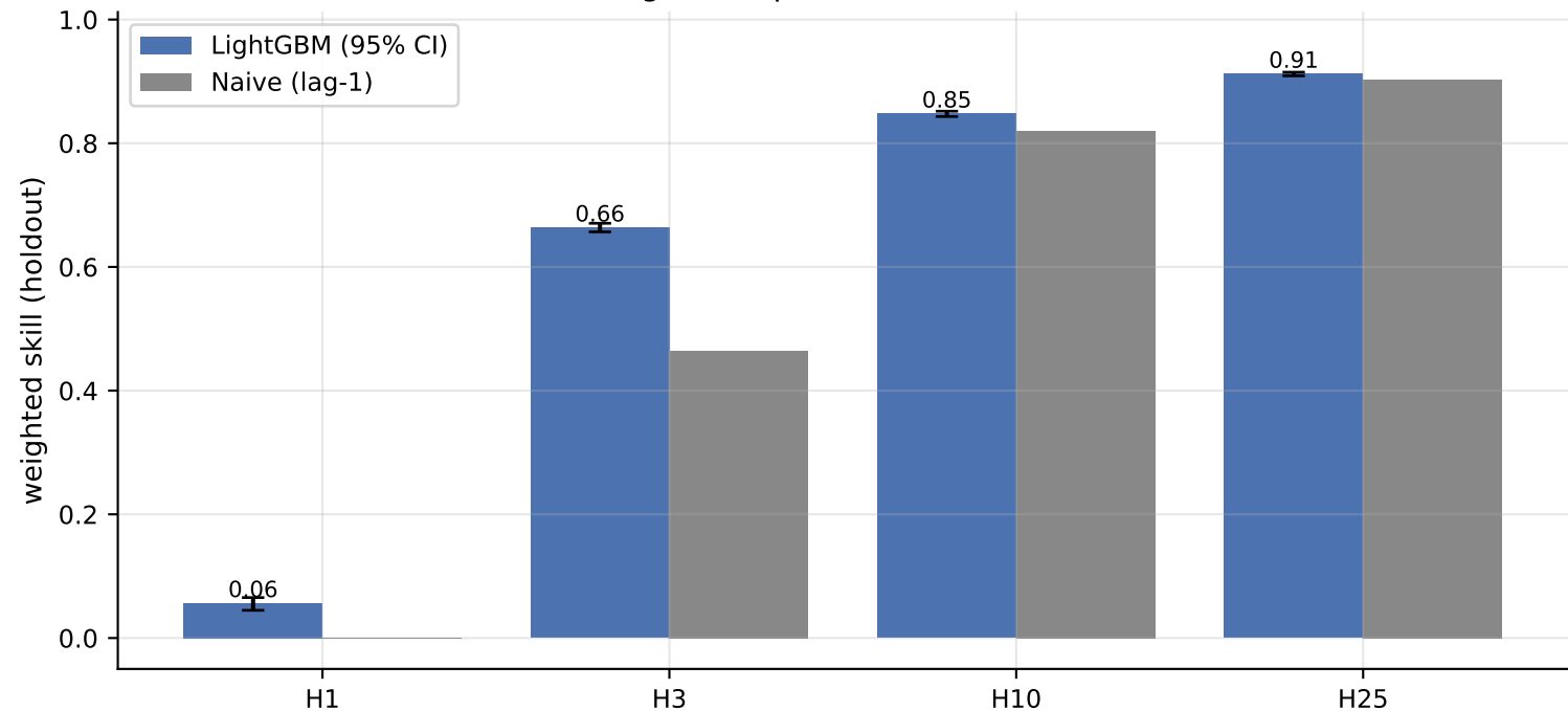
Global LightGBM per horizon, vs Naive floor
