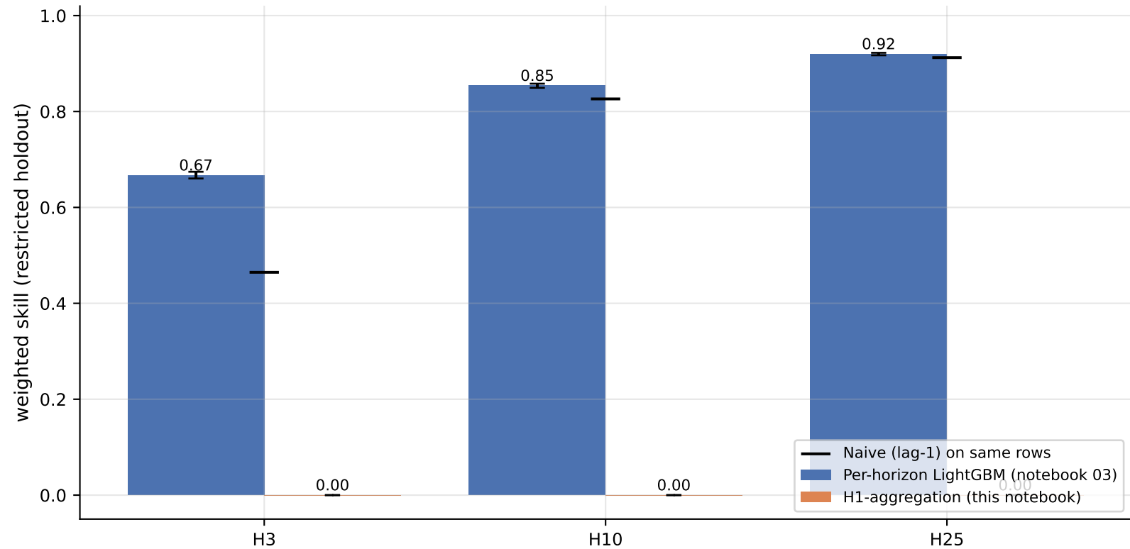
Per-horizon LGBM vs H1-aggregation, on identical rows
