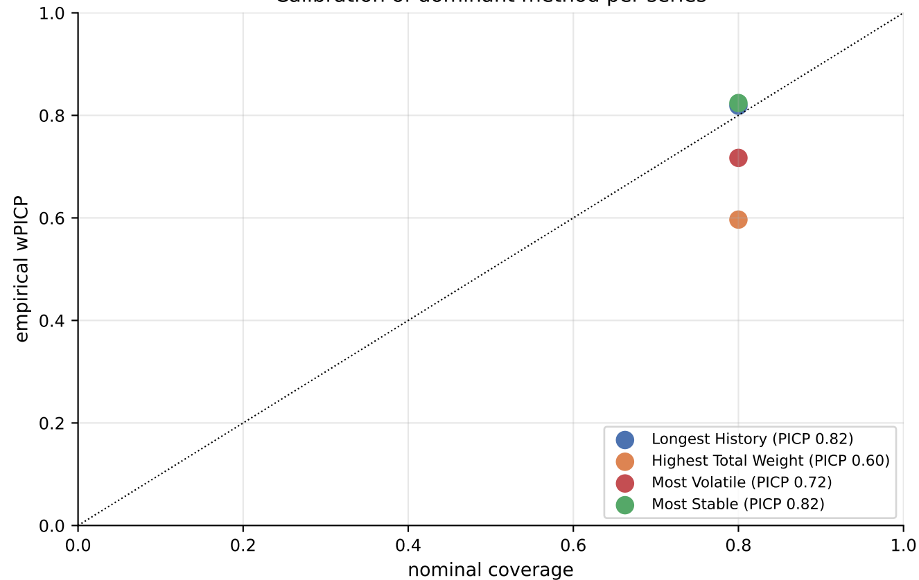
Calibration of dominant method per series
