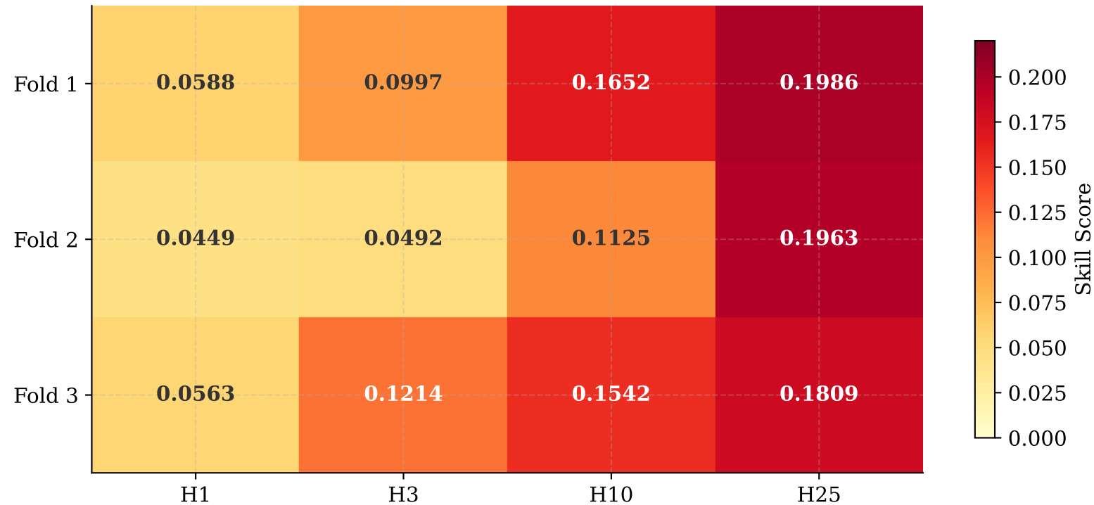
Weighted Skill Score — Fold x Horizon
