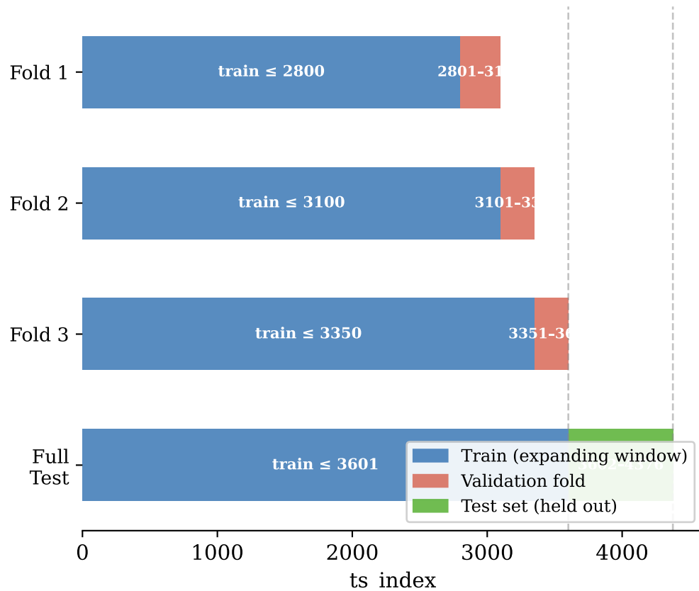
Expanding-Window Time-Based K-Fold
