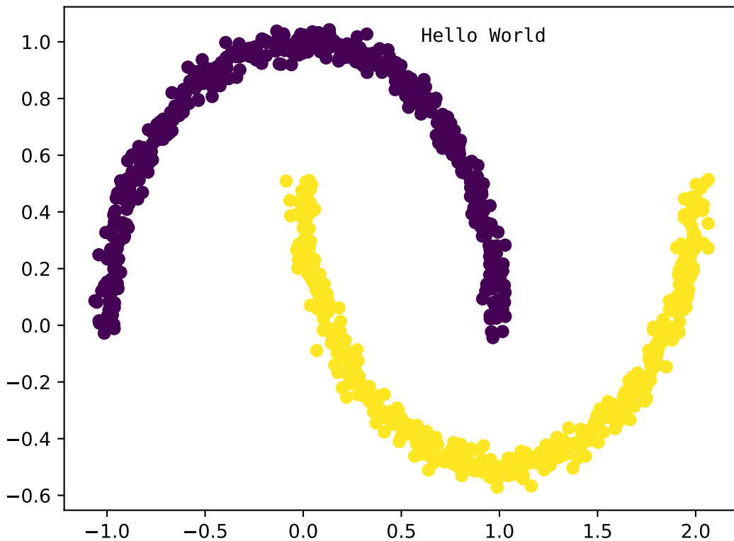
Scatter Plot
