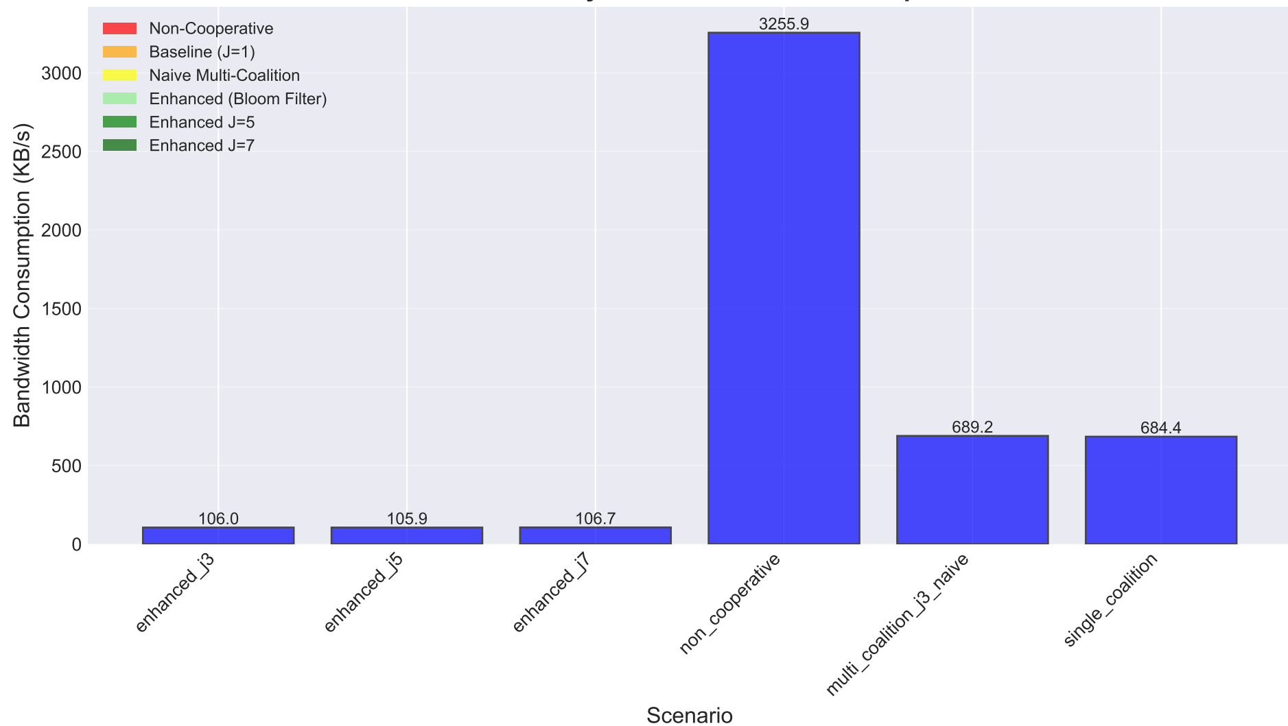
Bandwidth Efficiency: Naive vs Bloom Filter Optimization
