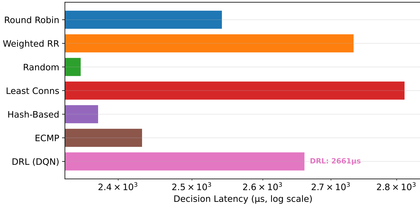
Decision Overhead per Algorithm
