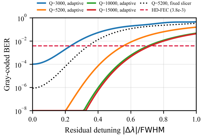
Fig. 1. Gray-coded BER versus residual resonance detuning for 100 GHz WDM and 25 dB electrical slicer SNR under identical Lorentzian-only receiver assumptions. Solid curves use adaptive mean-pedestal tracking; the dotted curve shows the conservative Q=5200 fixed-threshold receiver.
