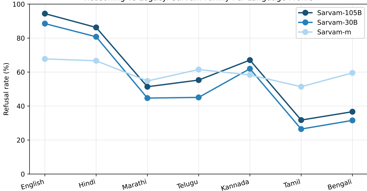
Reasoning vs Legacy: Sarvam Family Per-Language Profile
