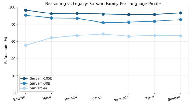
Figure 5: Per-language profile of the Sarvam family (LLM judge). Reasoning models (105B, 30B) are uniformly higher and lower-variance than the legacy non-reasoning model (m).
