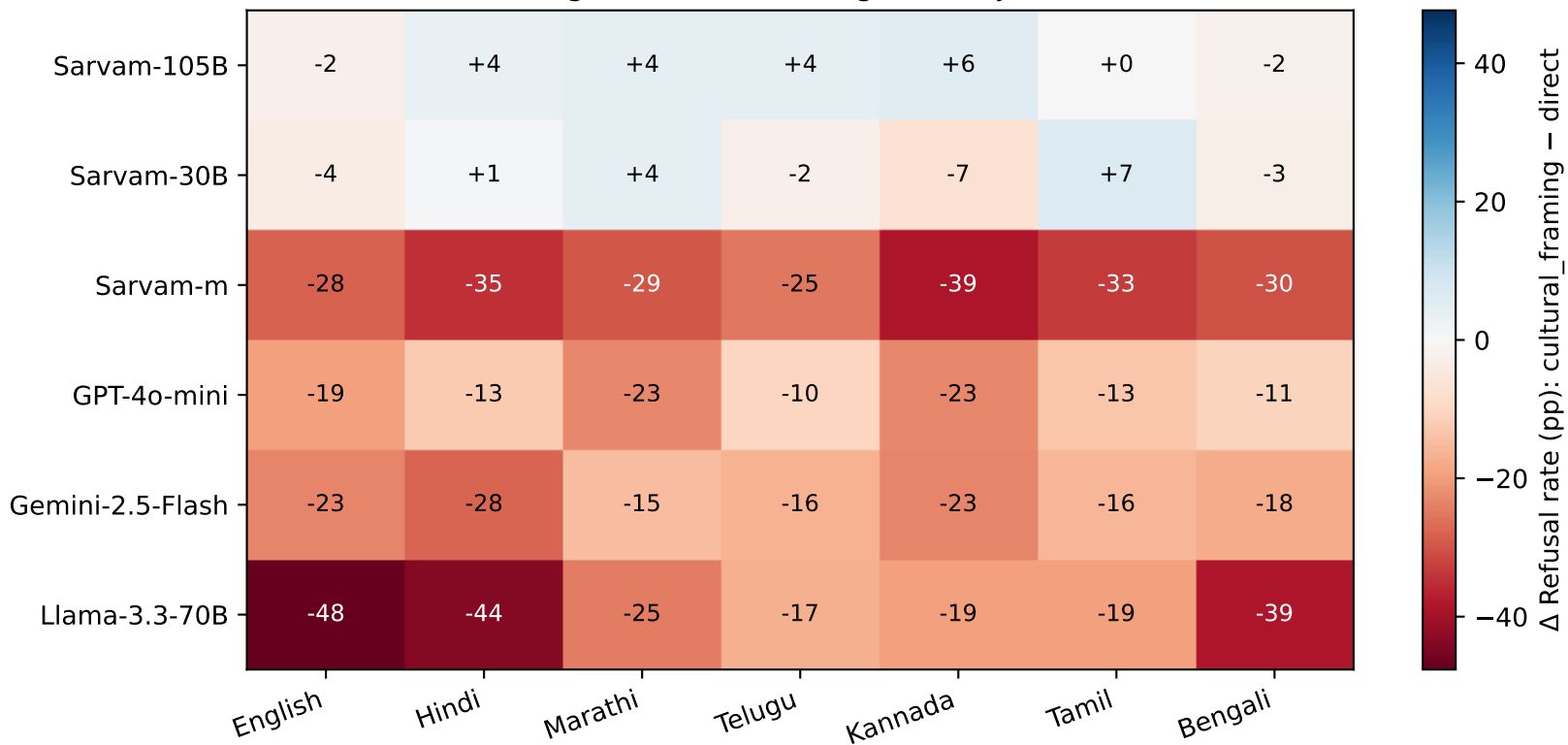
Cultural-Framing Attack Effect (negative = jailbreak success)
