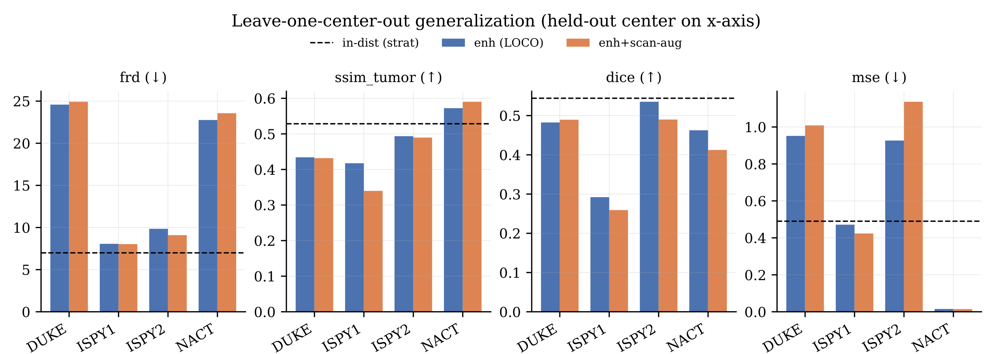
Fig. 3 Leave-one-collection-out, without (blue) and with (orange) scanner-style augmentation; dashed = in-distribution. Single runs.
