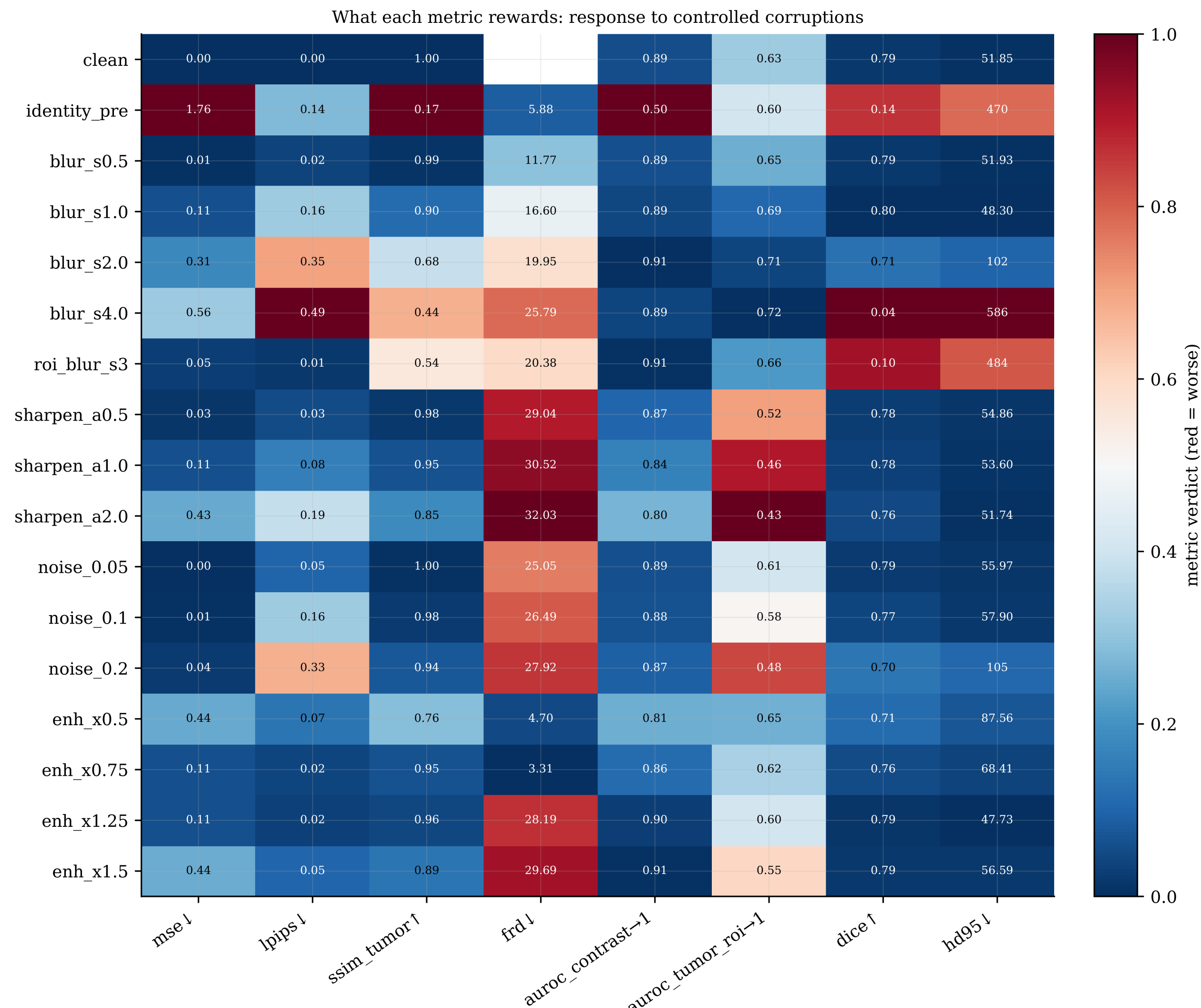
Fig. 4 Ground-truth images corrupted in controlled ways and re-scored by the official pipeline; red = judged worse. Single pass, 150 images.
