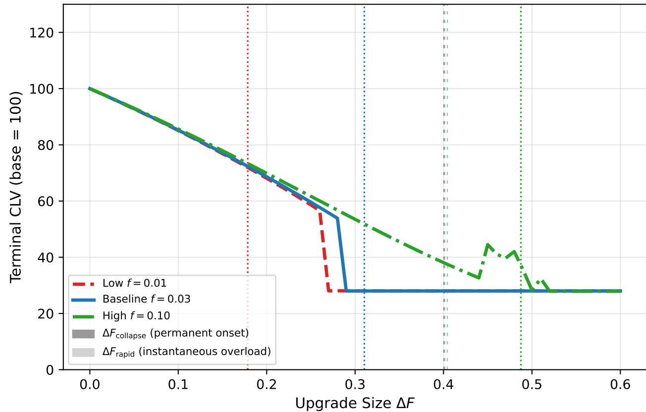
The Burnout Cliff \Delta F_{\text{collapse}} is workforce-contingent; \Delta F_{\text{rapid}} marks rapid-collapse onset
