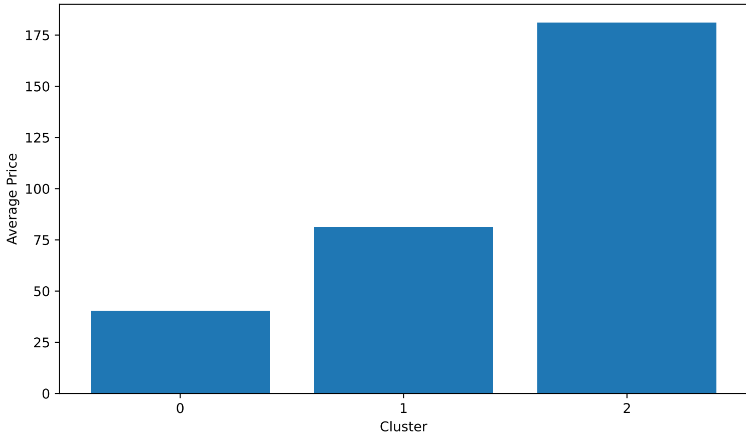
Product Clustering
