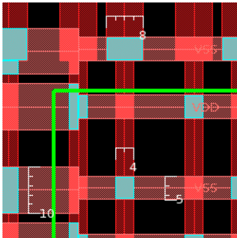
Figure 102 Tapering Straps
