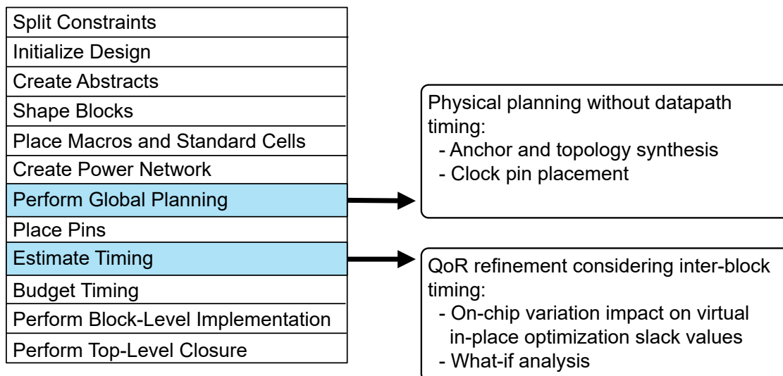
Figure 132 Clock Trunk Planning in the Overall Design Planning Flow
