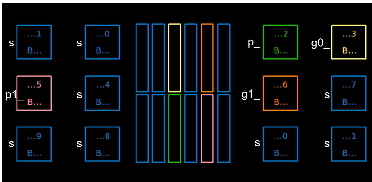
Figure 33 Bump Pattern With Three Rows
