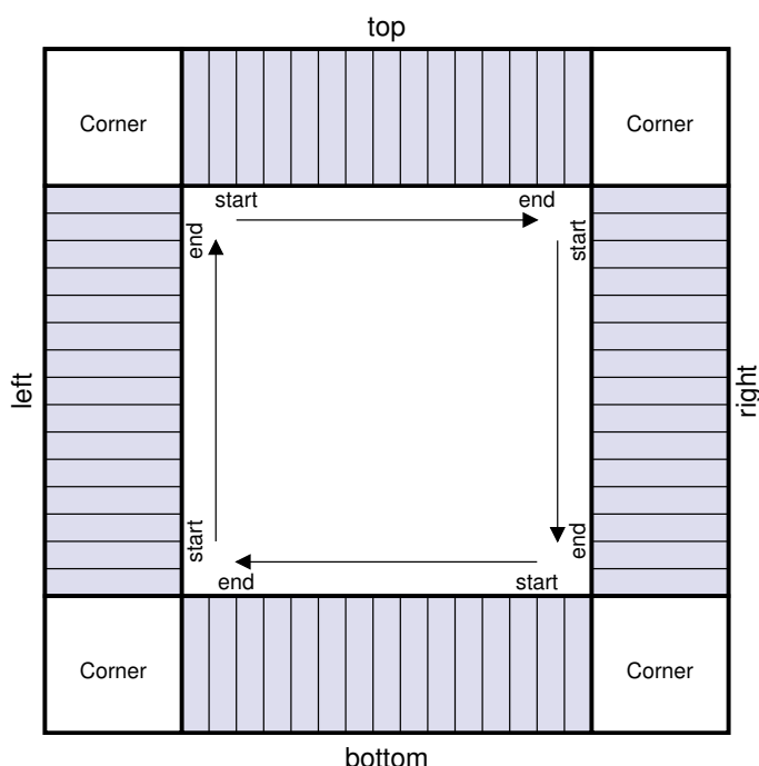
Figure 35 Signal I/O Constraints Side Ordering
