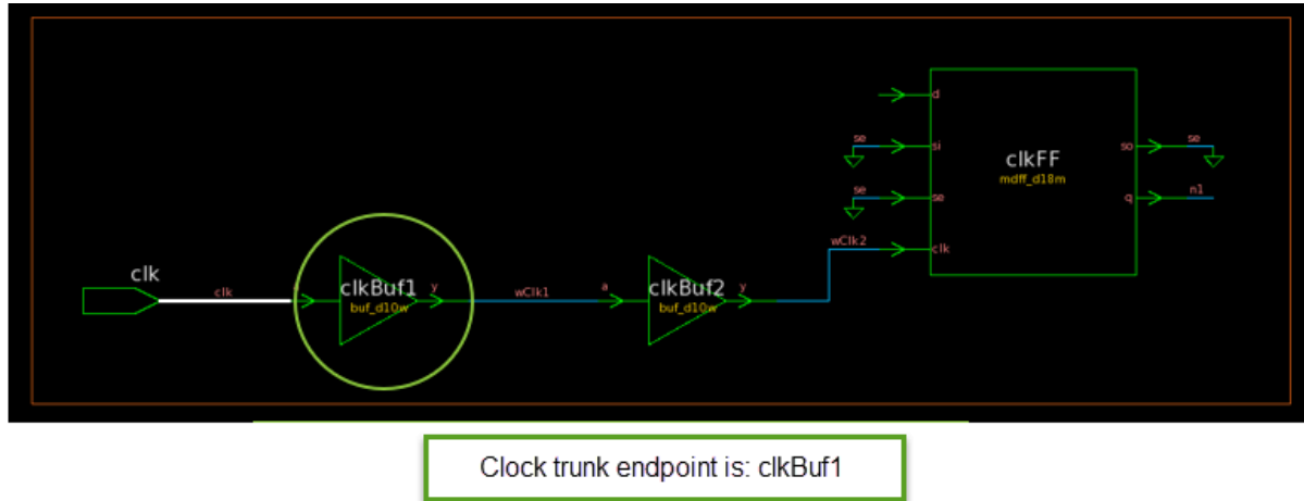
Figure 136 Clock to Single Flip-Flop With Buffers
