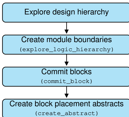
Figure 65 Manage Block Flow
