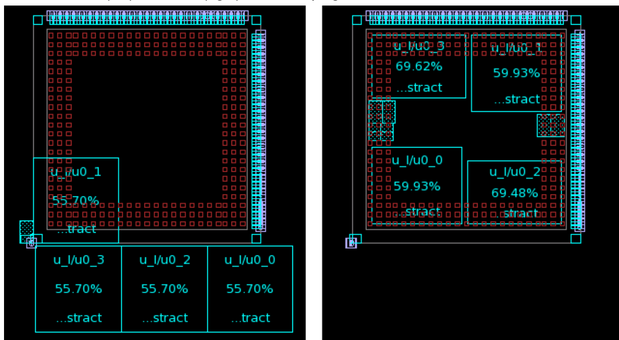
Figure 75 Before (left) and After (right) Block Shaping
