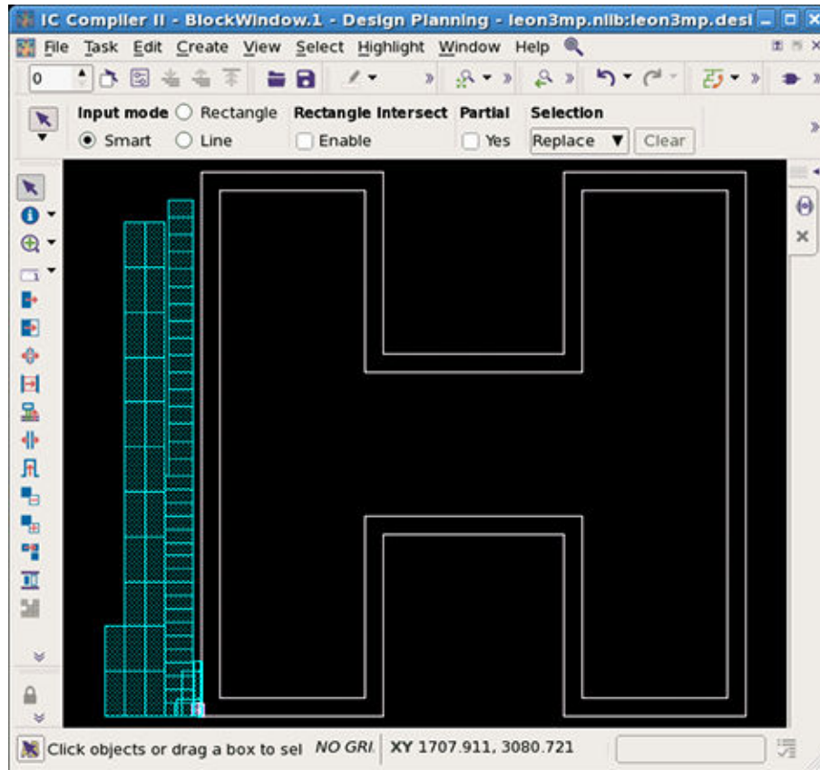
Figure 17 Complex Rectilinear Floorplan
