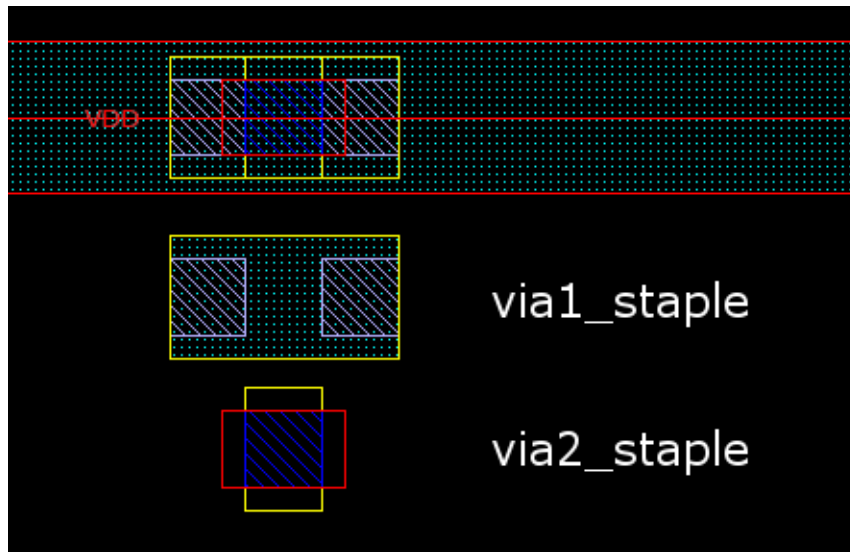
Figure 113 Stapling Via With Multiple Masters
