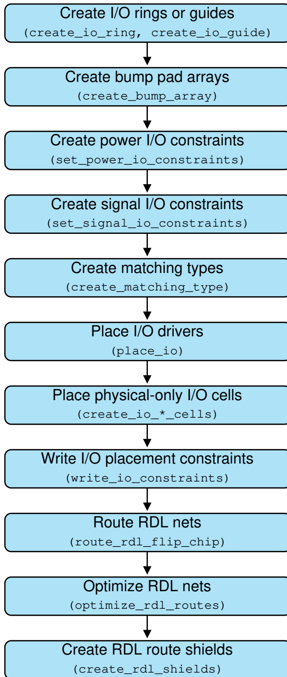
Figure 27 I/O Planning Flow
