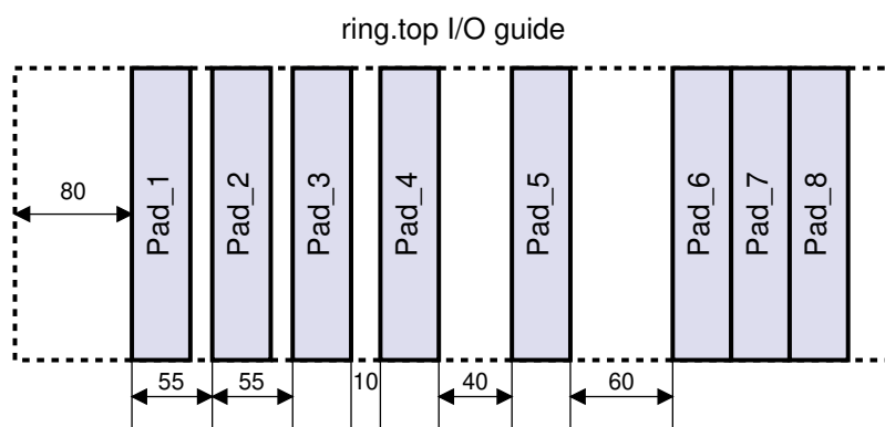
Figure 36 ring.top I/O Placement
