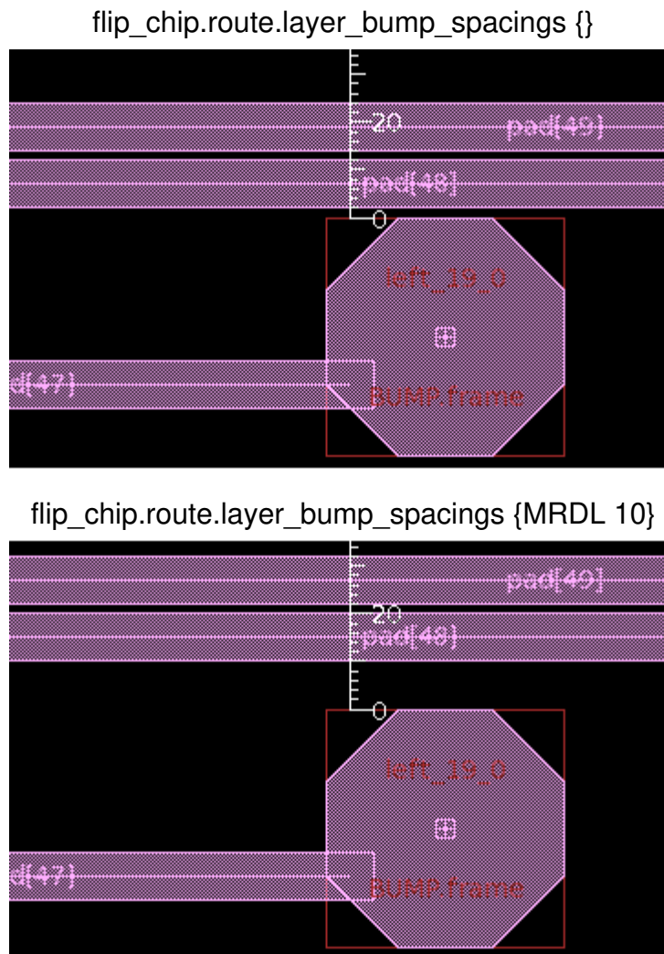
Figure 50 Bump-to-Route Spacing
