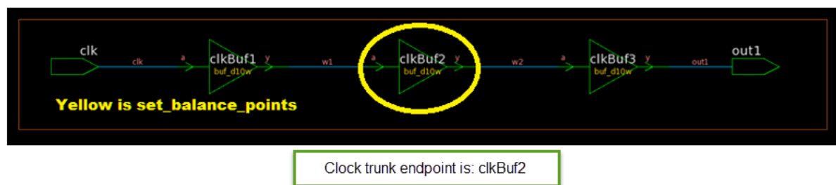
Figure 142 Buffered Feedthrough With Balance Point on One Buffer
