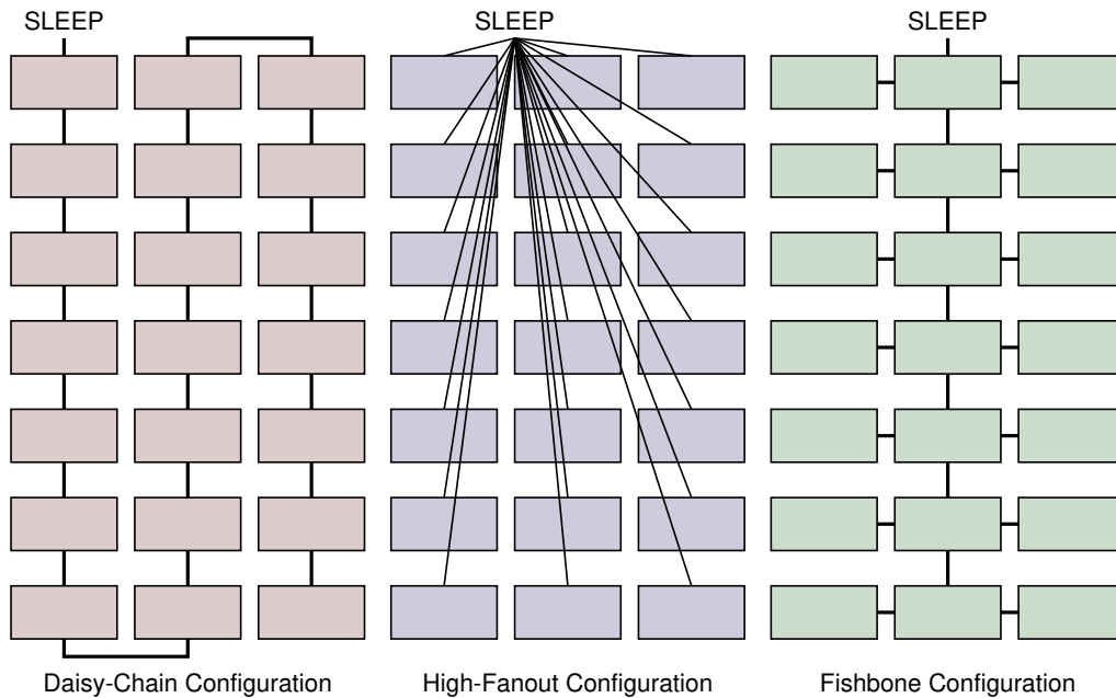
Figure 114 Power Switch Fanout Configurations
