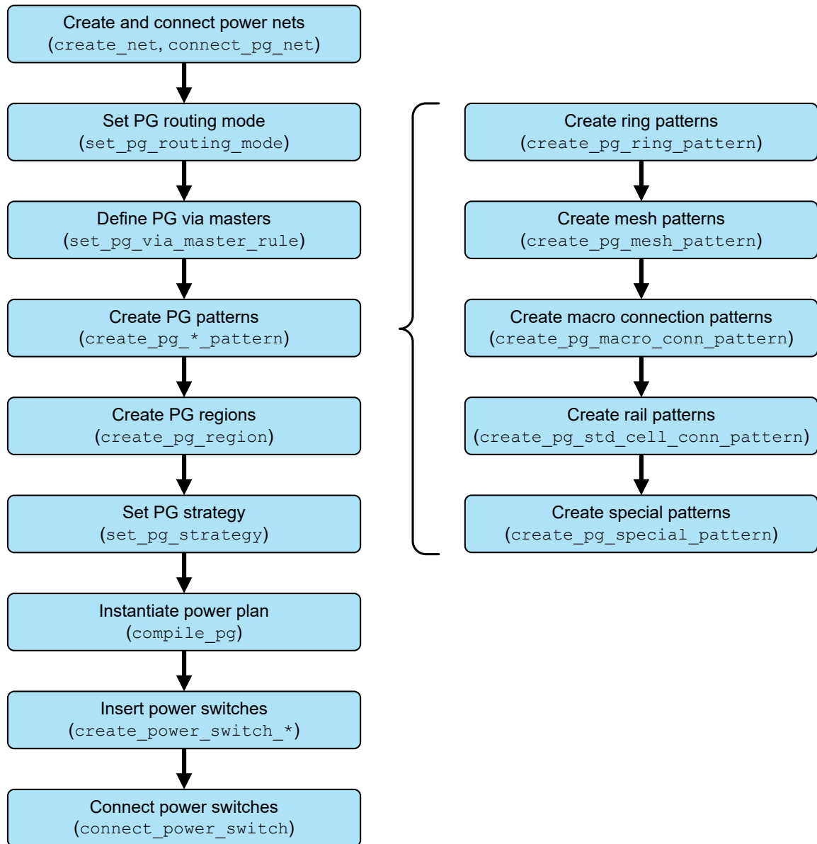
Figure 94 Pattern-Based Power Planning Flow
