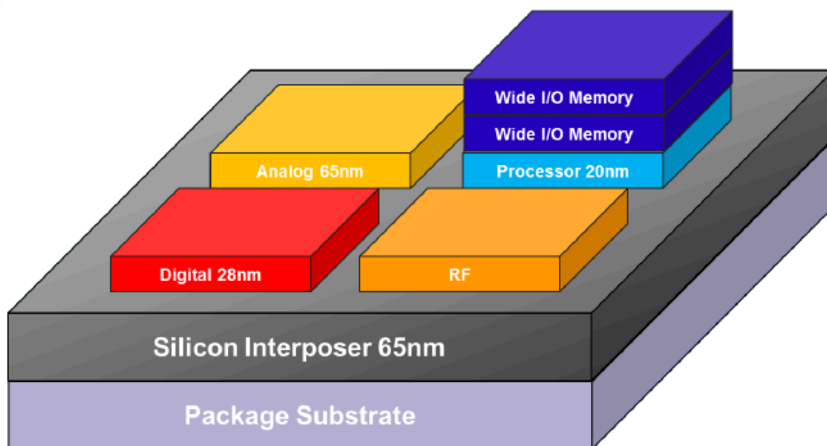
Figure 58 Complex 3DIC Design
