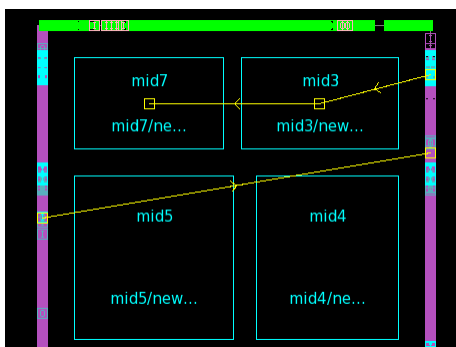
Figure 119 Topology Plans With and Without Feedthroughs
