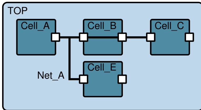
Figure 149 Topological Constraints Example 2
