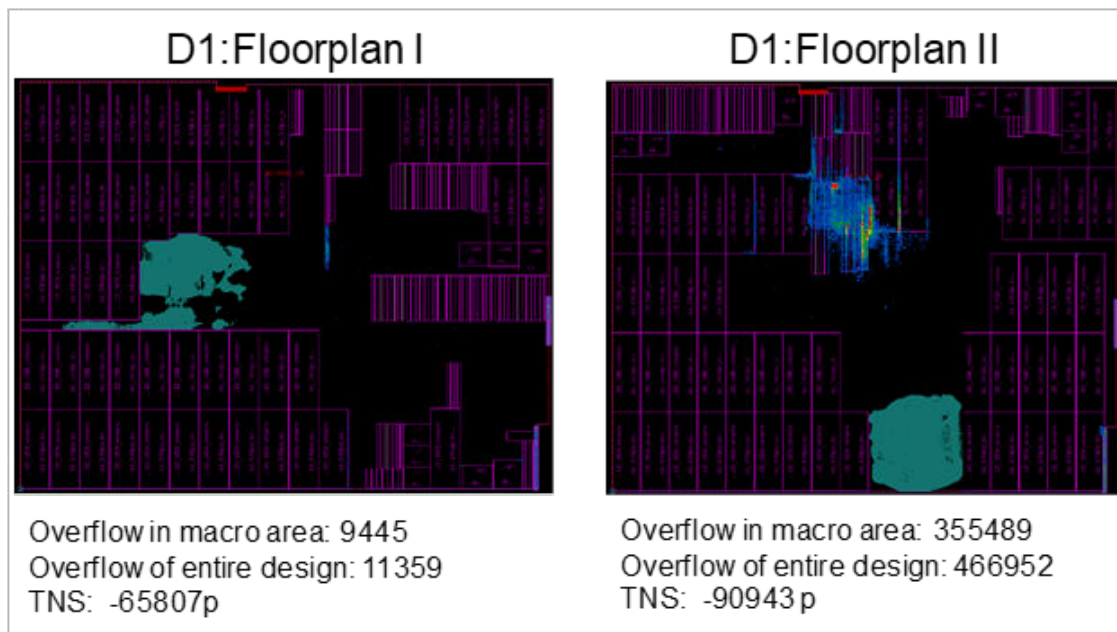
Figure 86 Different Floorplans as a Result of Different Macro Placements
