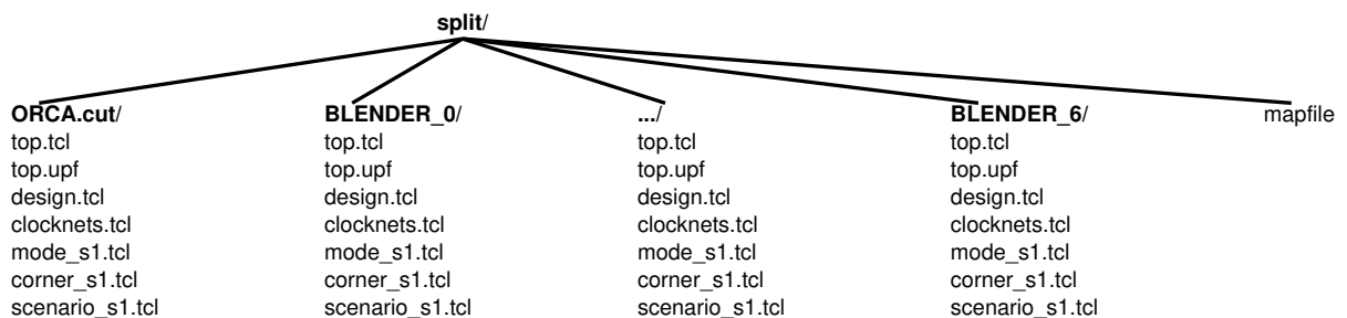
Figure 8 Constraint Files After split_constraints
