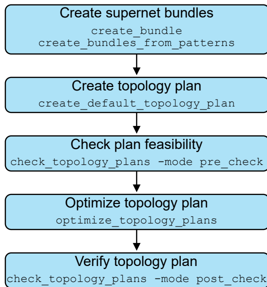
Figure 118 Topology Interconnect Planning Flow
