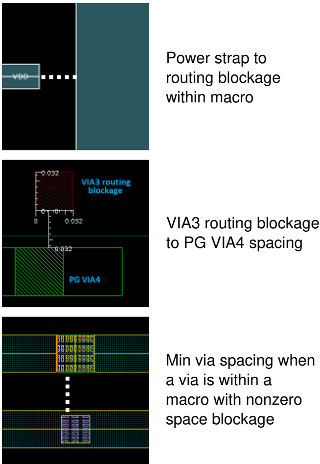
Figure 109 Minimum Spacing Violations to Blockages
