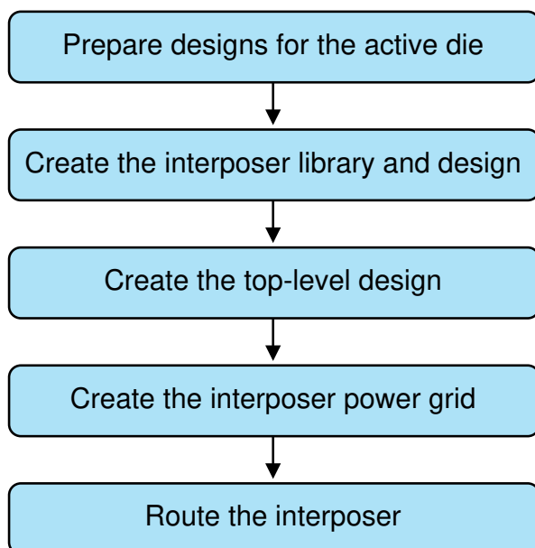
Figure 59 3DIC Flow for 2.5D Design
