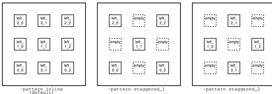
Figure 30 Bump Array Placement Pattern Options
