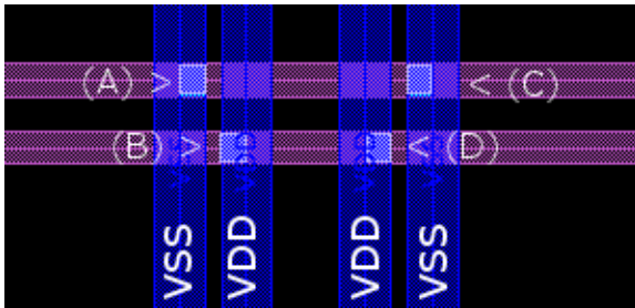
Figure 96 Annotated Center-Aligned Vias
