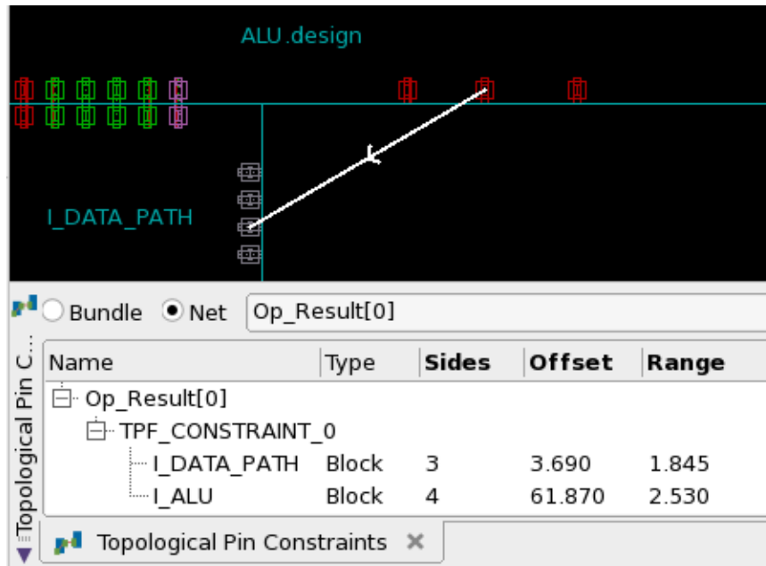
Figure 162 Pin Placement Result After Defining a Topological Constraint
