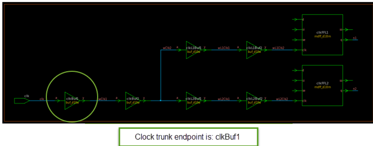
Figure 137 Clock to Multiple Flip-Flops With Buffers on Common Path
