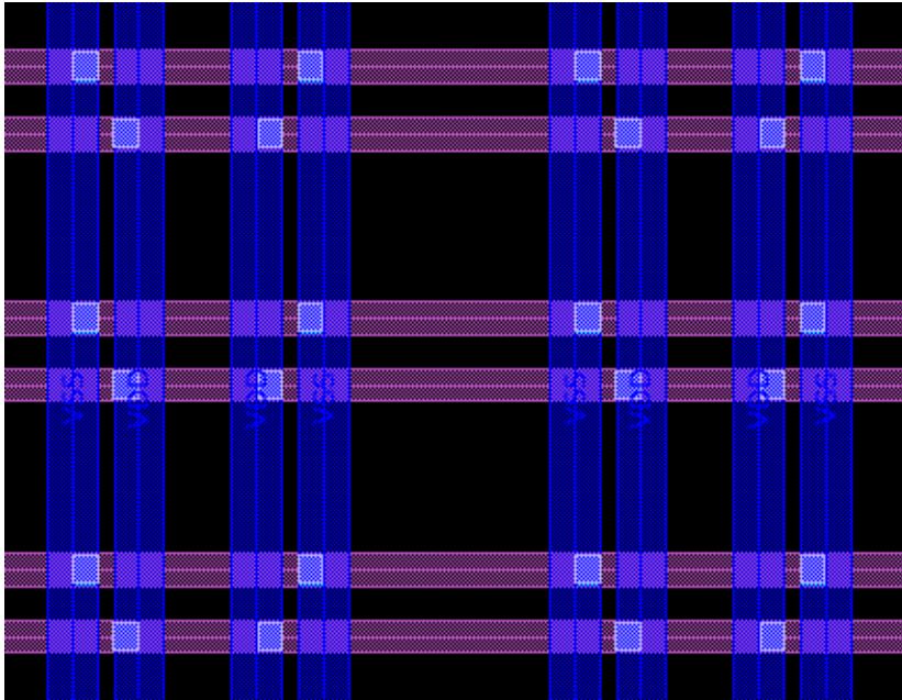
Figure 95 Power Straps With Center-Aligned Vias
