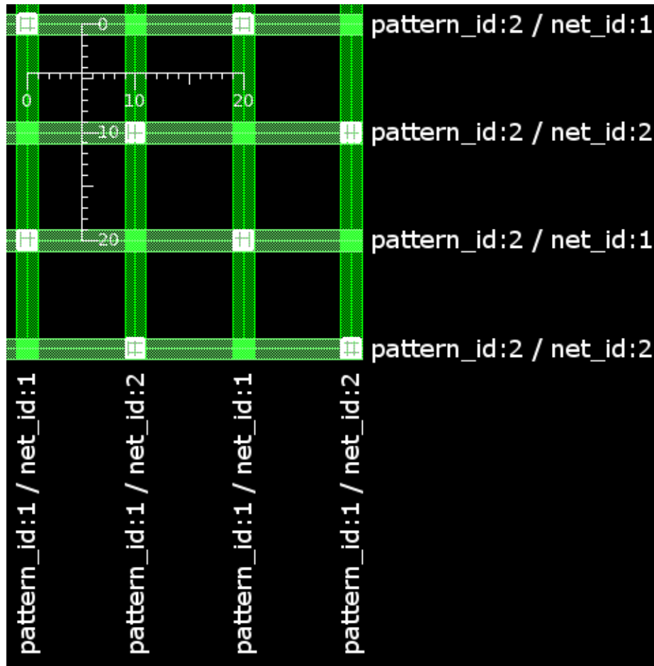
Figure 105 Annotated Checkerboard Pattern
