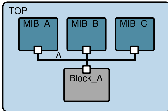
Figure 156 Topological Constraints for Multiply Instantiated Blocks
