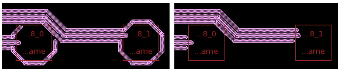
Figure 55 Bump Shields -shield_on_bump Option
