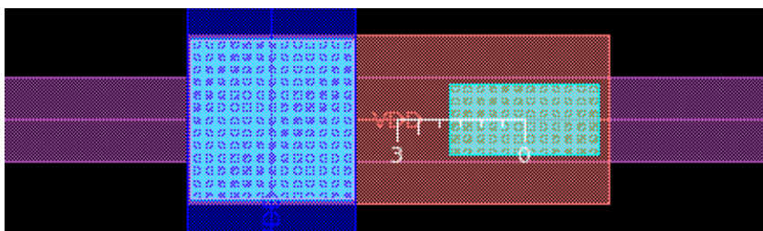
Figure 101 Via Offset From Center
