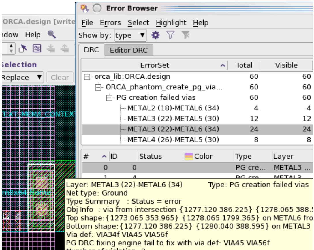
Figure 110 Phantom Via
