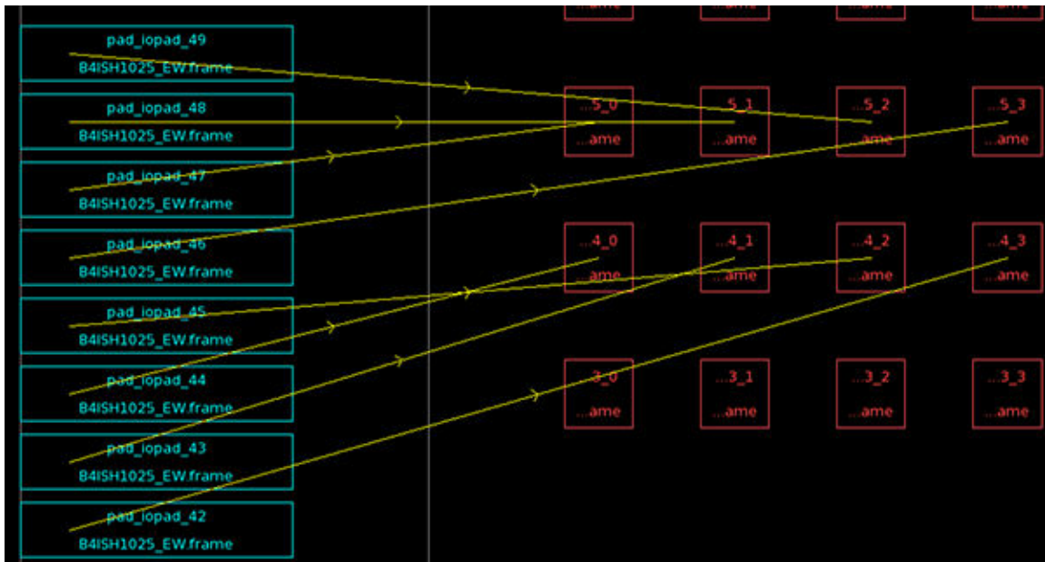
Figure 39 RDL Flylines Between Matching Cells
