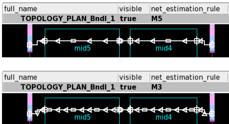
Figure 126 Optimizing Topology Plans for Different Net Estimation Rules
