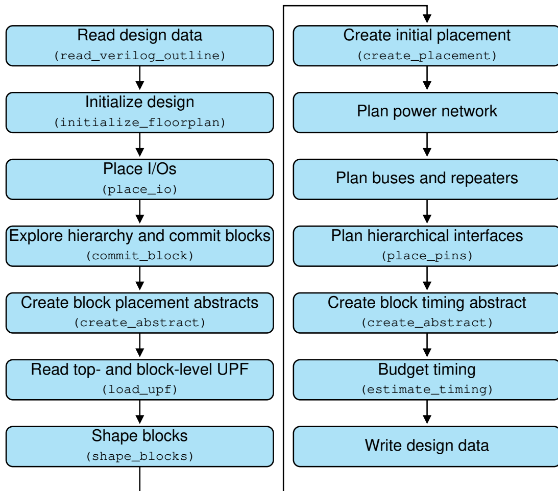
Figure 1 Hierarchical Design Planning Flow
