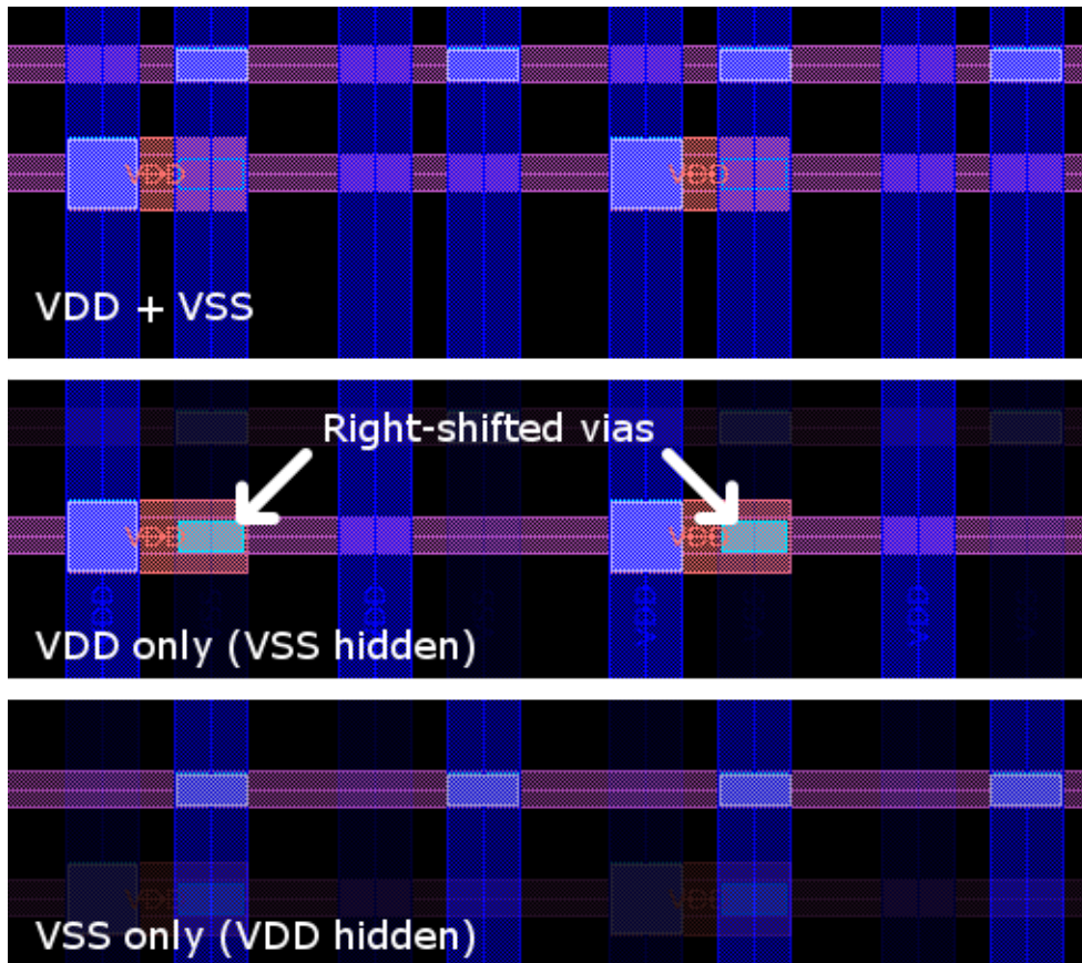
Figure 100 Composite Bridging Pattern Structure
