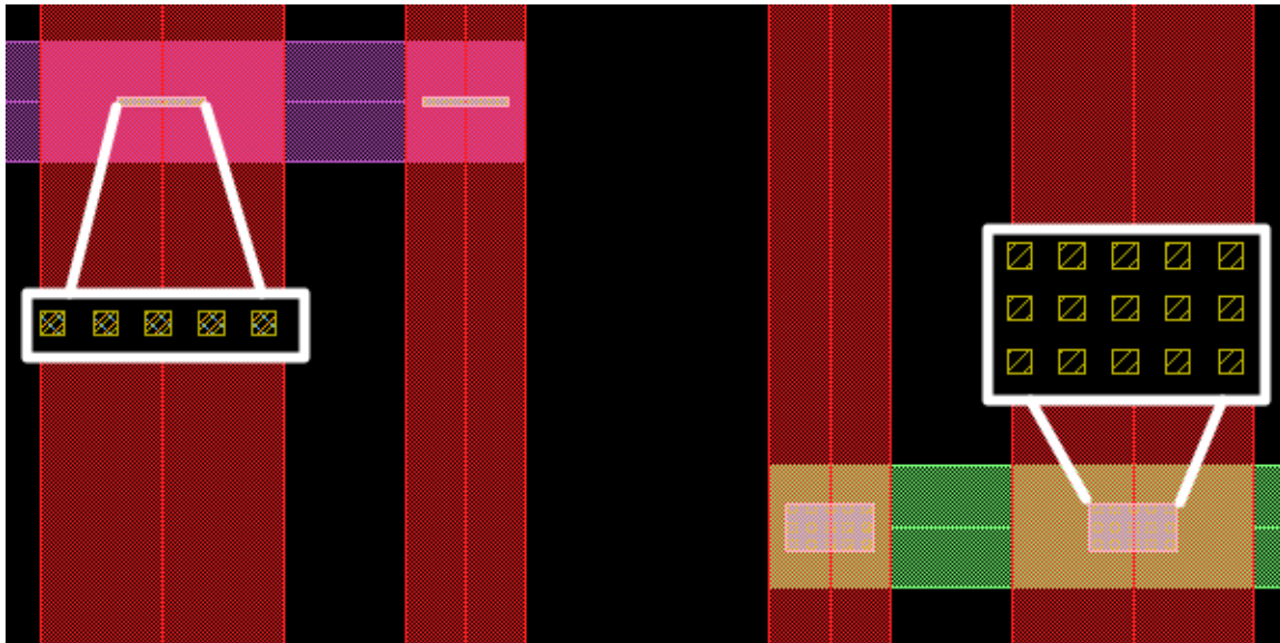
Figure 98 5x1 and 5x3 Vias
