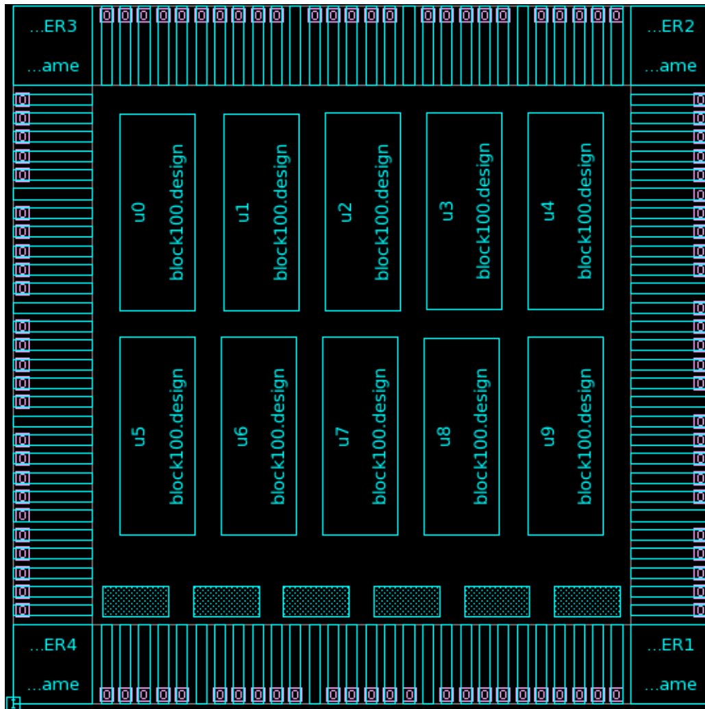
Figure 76 Layout With Shaping Constraints
