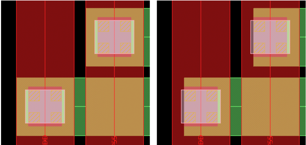
Figure 116 Trim to Wire and Trim to Via
