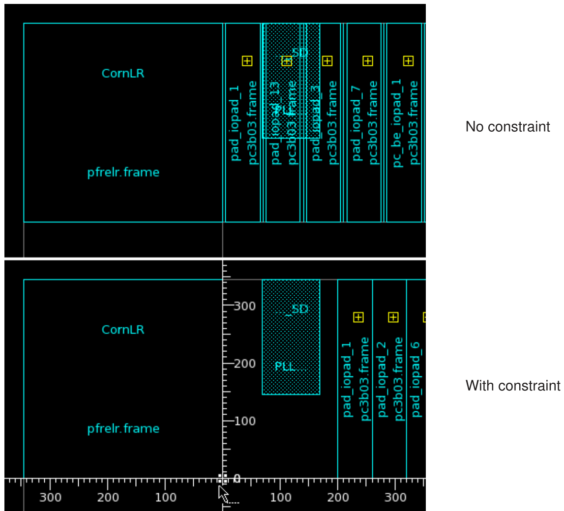
Figure 37 place_io Fixed Pad Constraint Comparison
