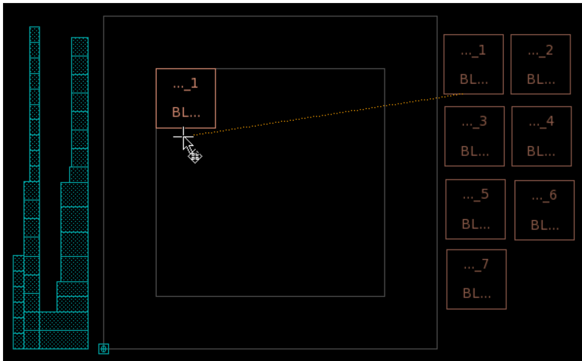
Figure 68 Moving Module Boundaries
