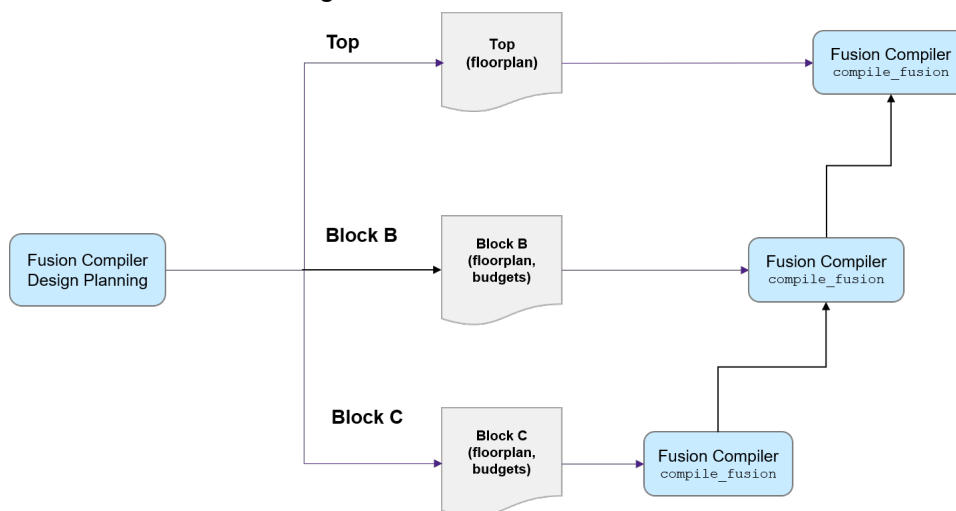
Figure 166 Traditional Design Flow
