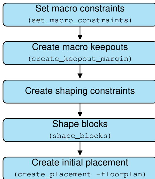
Figure 72 Block Shaping Flow
