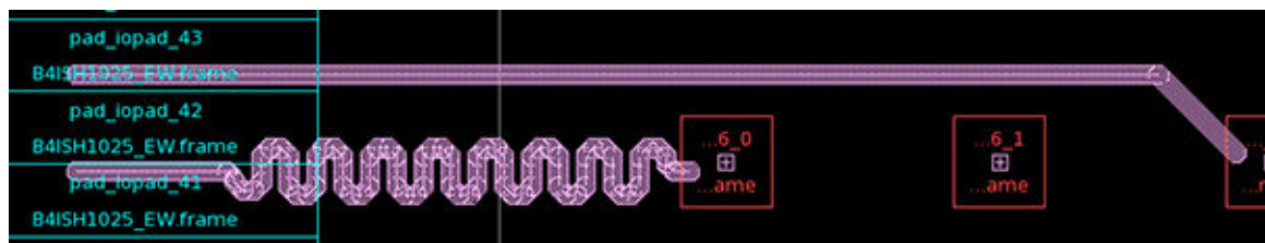
Figure 44 Differential Routes
