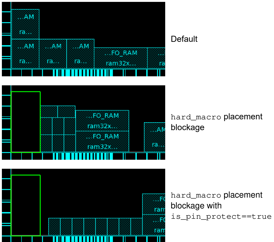
Figure 85 Macros Placed Away From Block Edges
