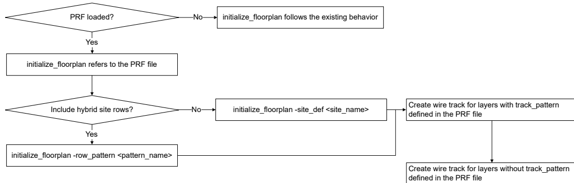
Figure 18 Example - Physical Rule File Based Floorplan Creation Flow
