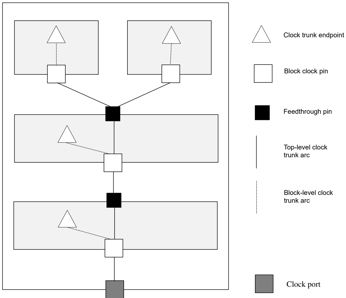
Figure 133 Clock Trunk Planning Terminology
