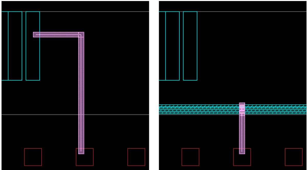
Figure 48 RDL Route to Pad and PG Stripe
