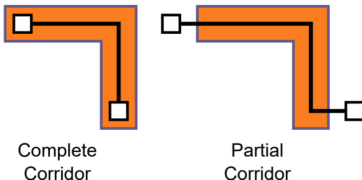
Figure 131 Complete and Partial Routing Corridors
