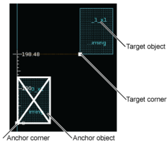
Figure 73 Macro Relative Location
