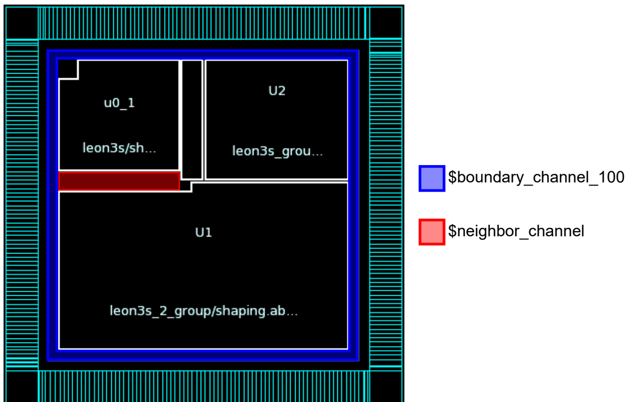
Figure 81 Block Shaping and Channel Constraints
