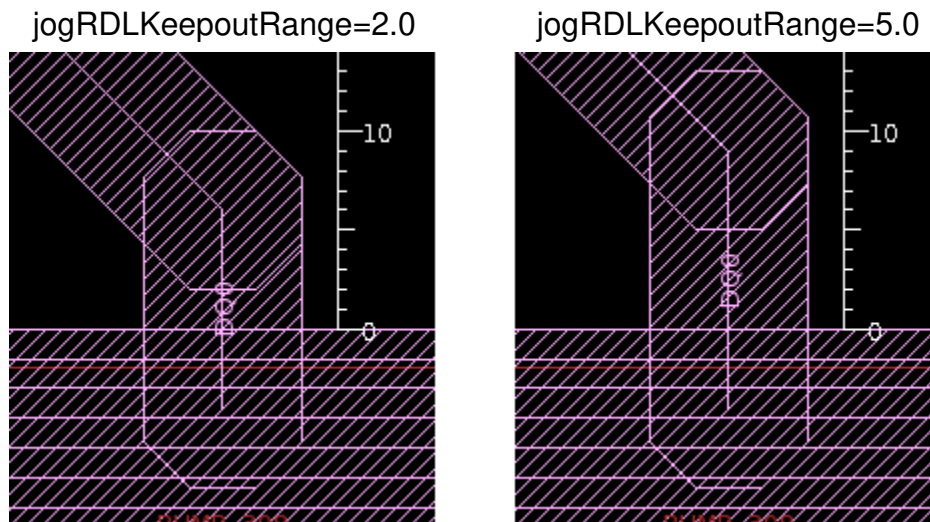
Figure 51 Jog Keepout Range
