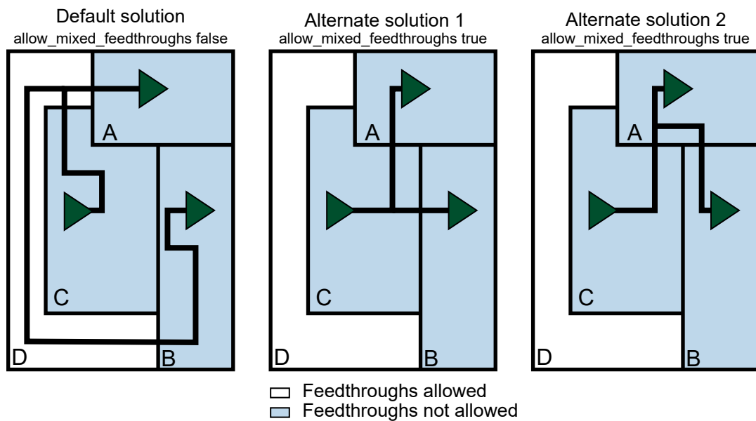
Figure 154 Mixed Feedthroughs in Disallowed Blocks
