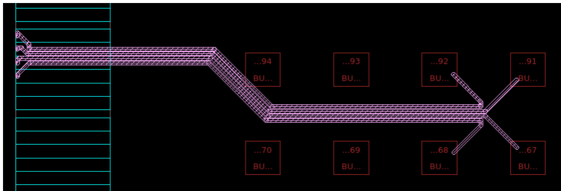
Figure 45 Differential Routes - Normal Mode
