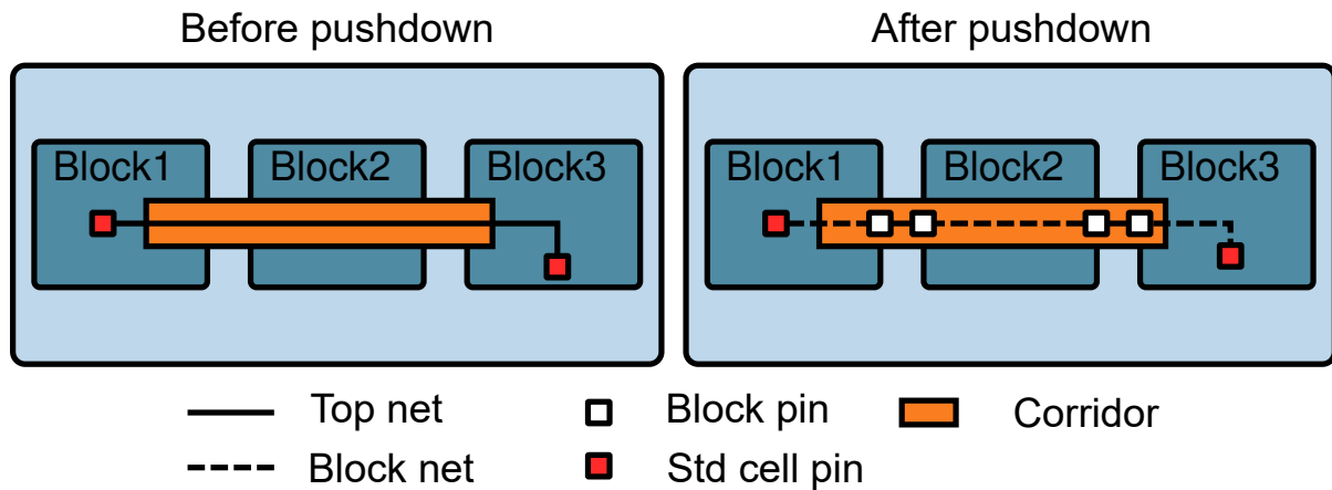
Figure 70 Pushdown Global Route
