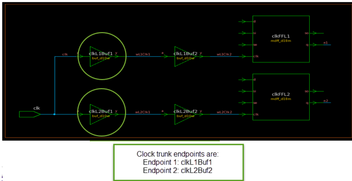
Figure 138 Clock to Multiple Flip-Flops With Buffers Only on Branch Path
