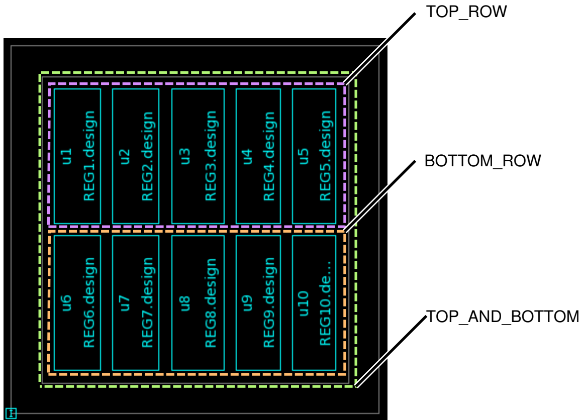
Figure 78 Block Shaping Example
