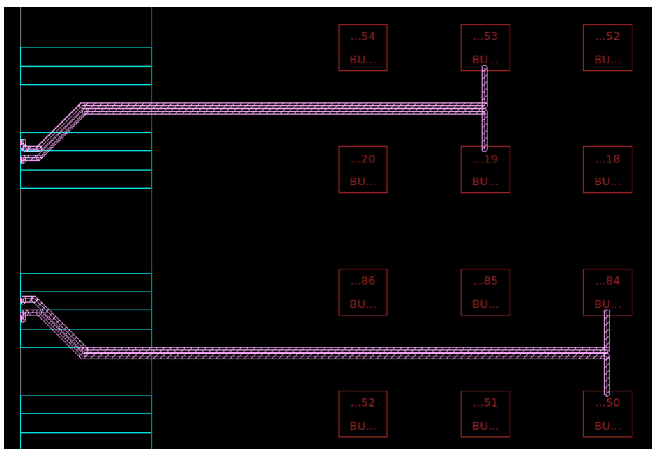
Figure 46 Differential Routes - Parallel Mode
