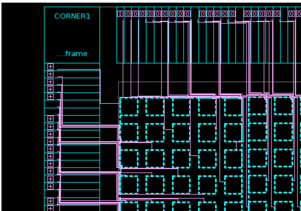
Figure 41 Layout After Flip-Chip Routing
