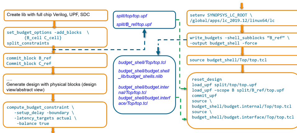
Figure 168 Budget Shell Flow for Multivoltage Designs
