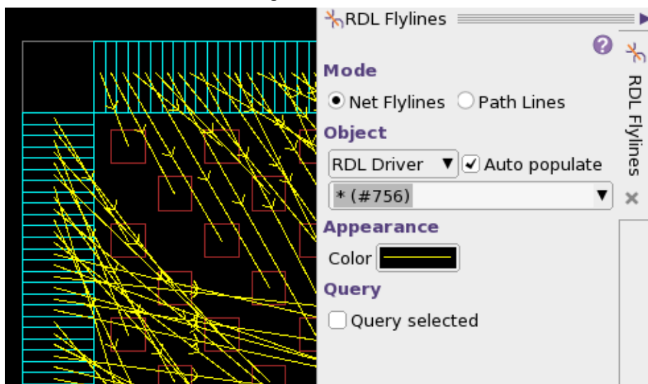
Figure 38 Default RDL Net Assignments
