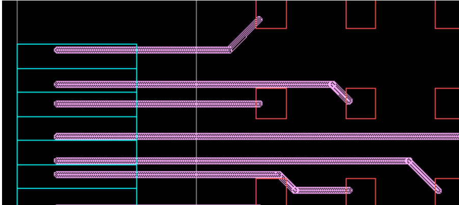
Figure 42 45-Degree RDL Routes
