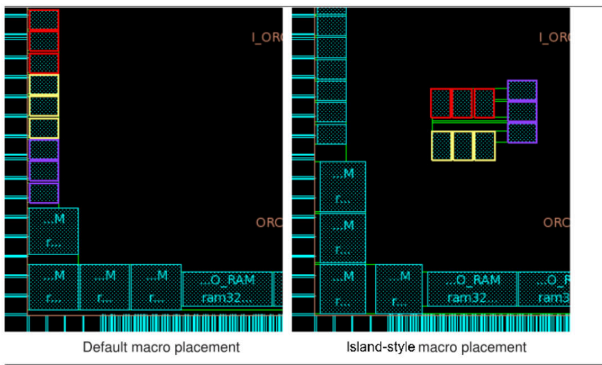
Figure 84 Default and Island Macro Placement
