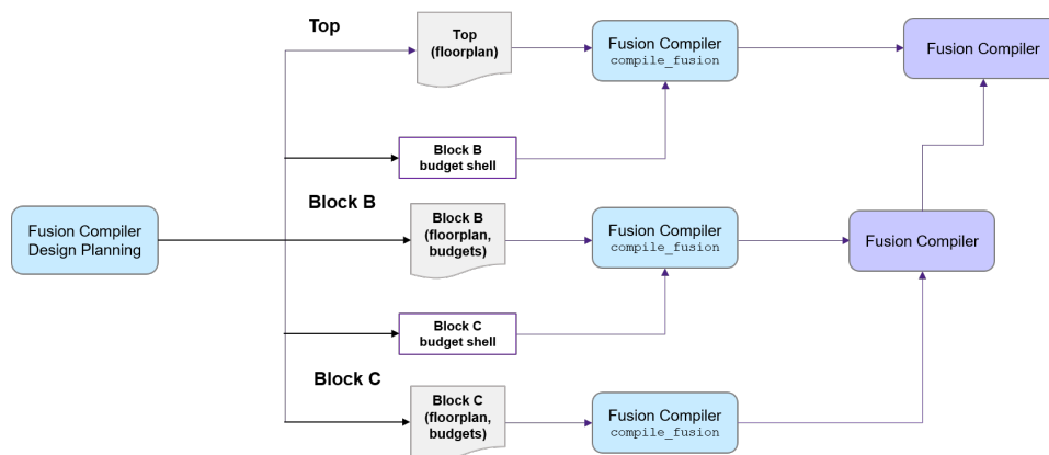
Figure 167 Hierarchical Design Flow
