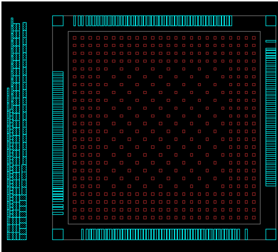
Figure 29 Layout After create_bump_array
