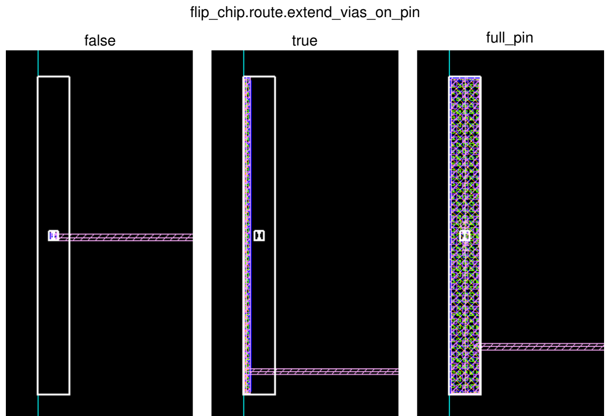
Figure 49 Additional Stacked Vias for RDL Routes to I/O Driver Pins
