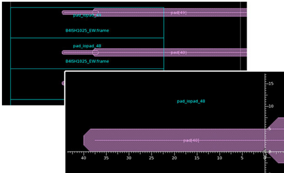
Figure 47 Tapered RDL Routes
