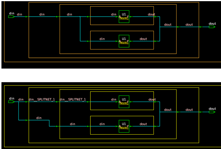
Figure 71 Before and After Pushing to the Top Level
