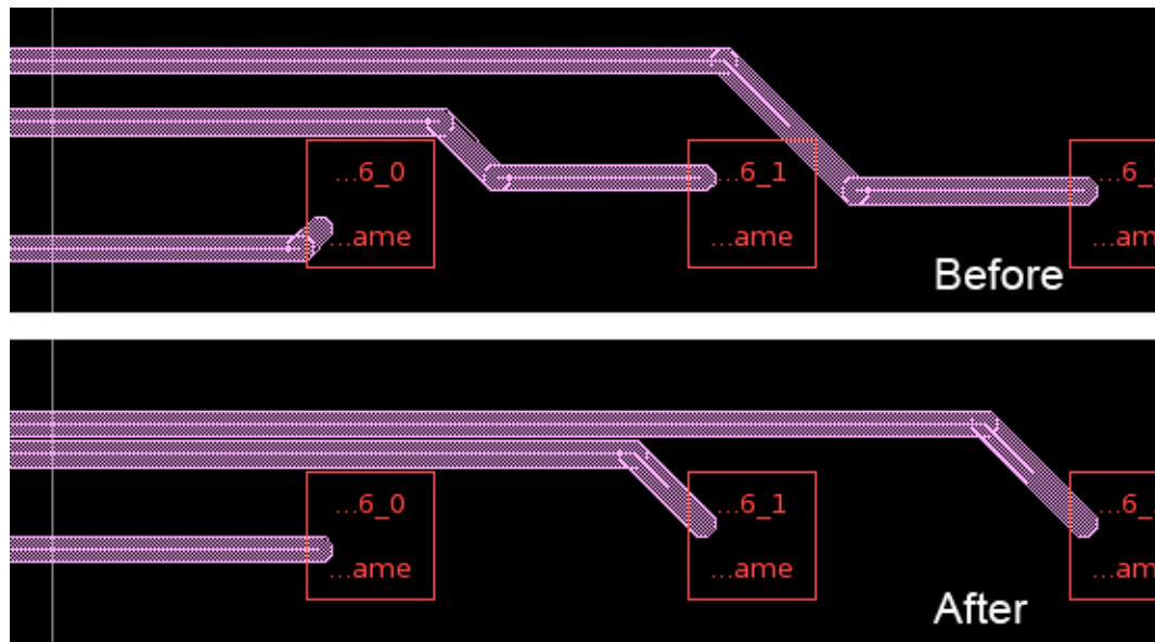
Figure 52 RDL Route Optimization
