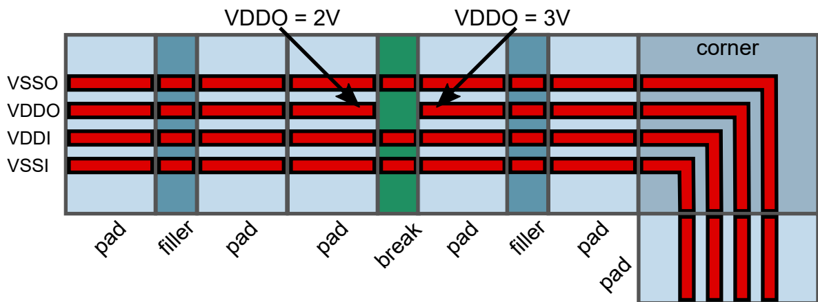
Figure 40 I/O Pad, Corner, Filler, and Break Cells
