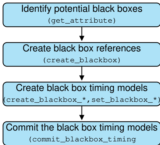
Figure 23 Black Box Flow
