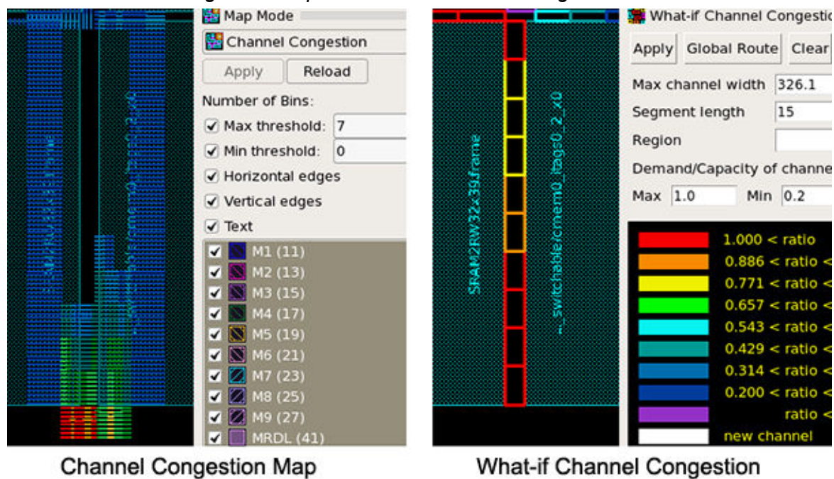
Figure 158 Channel Congestion Map and What-if Channel Congestion
