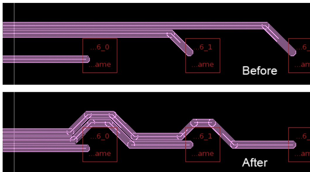
Figure 53 RDL Route Optimization to Reserve Power Resources
