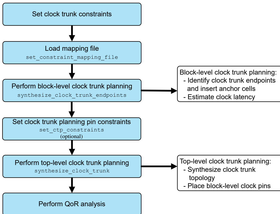
Figure 134 Clock Trunk Planning Flow
