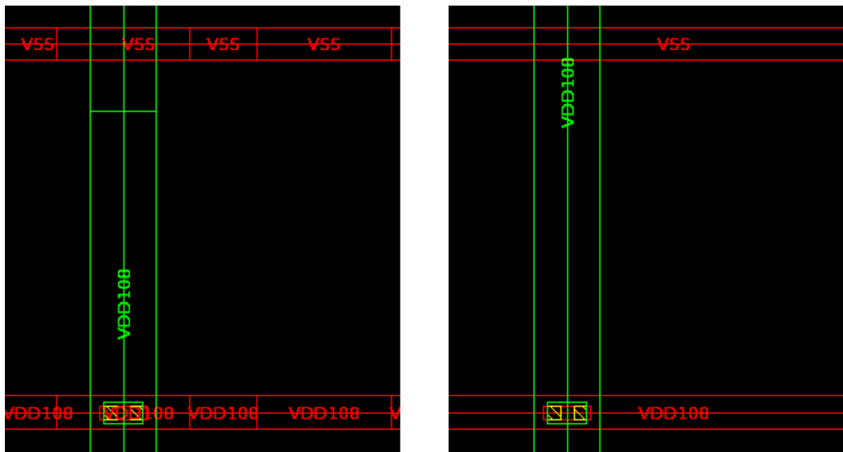
Figure 111 Before and After Merging Shapes in the PG Mesh
