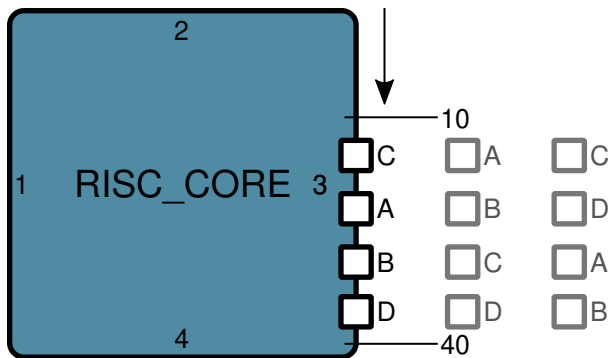
Figure 157 Physical Pin Constraint Example
