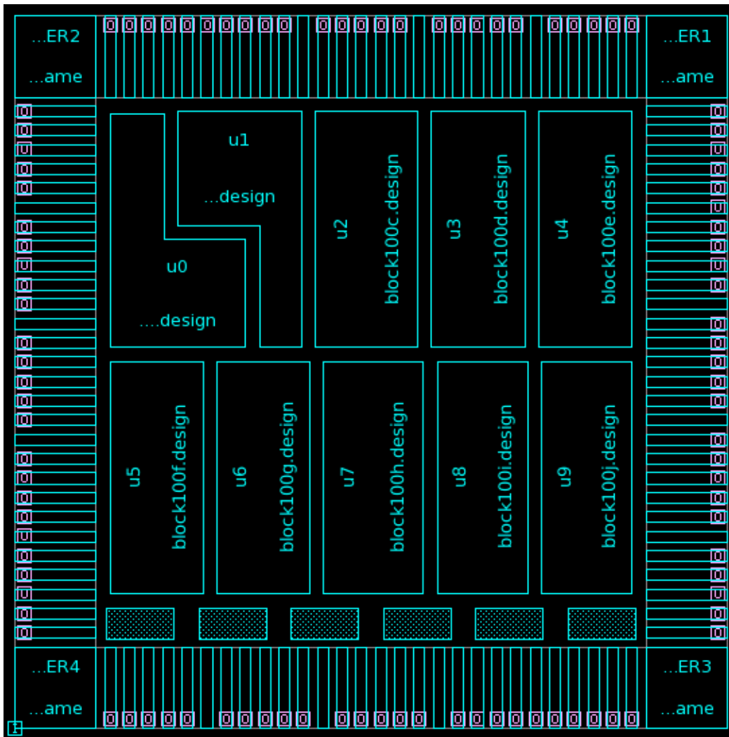
Figure 77 Layout With Fixed Boundary
