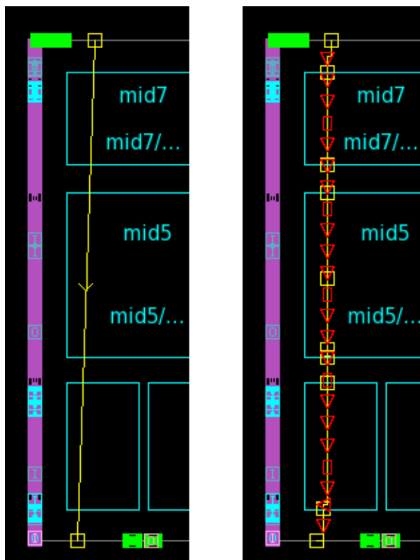
Figure 124 Optimize Topology Plan
