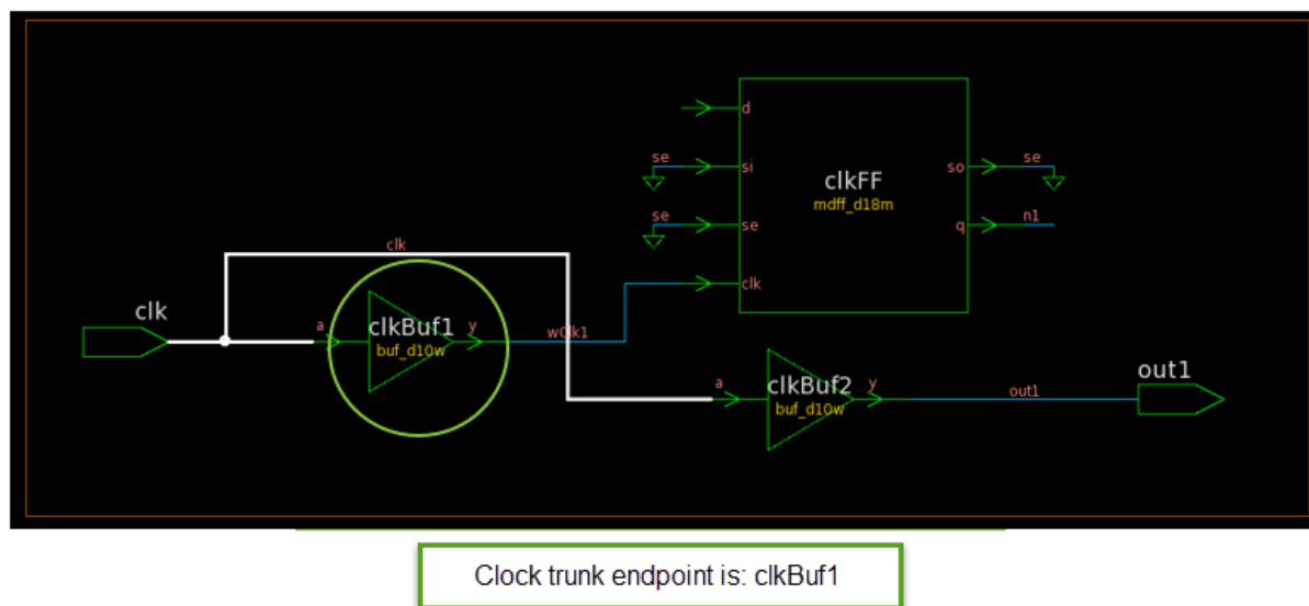
Figure 139 Clock to Flip-Flop With Buffers and Buffered Feedthrough
