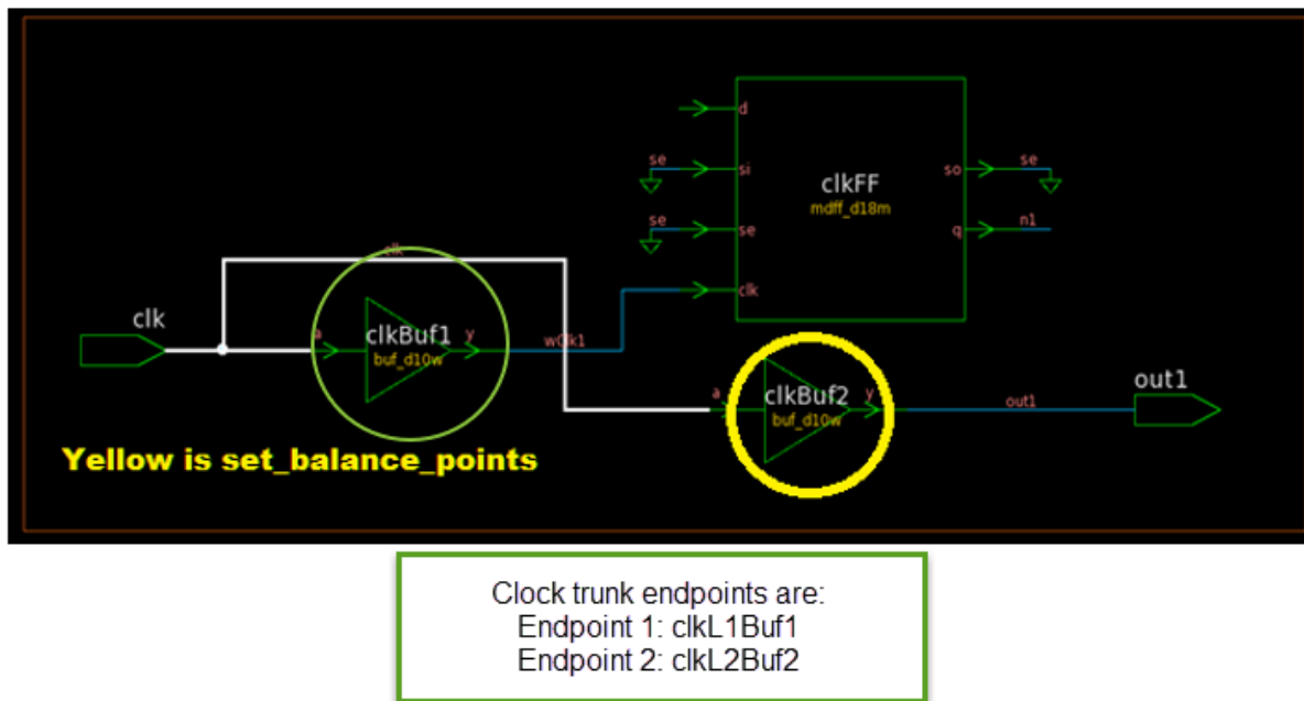
Figure 140 Clock to Flip-Flop With Buffers and Buffered Feedthrough With Balance Point
