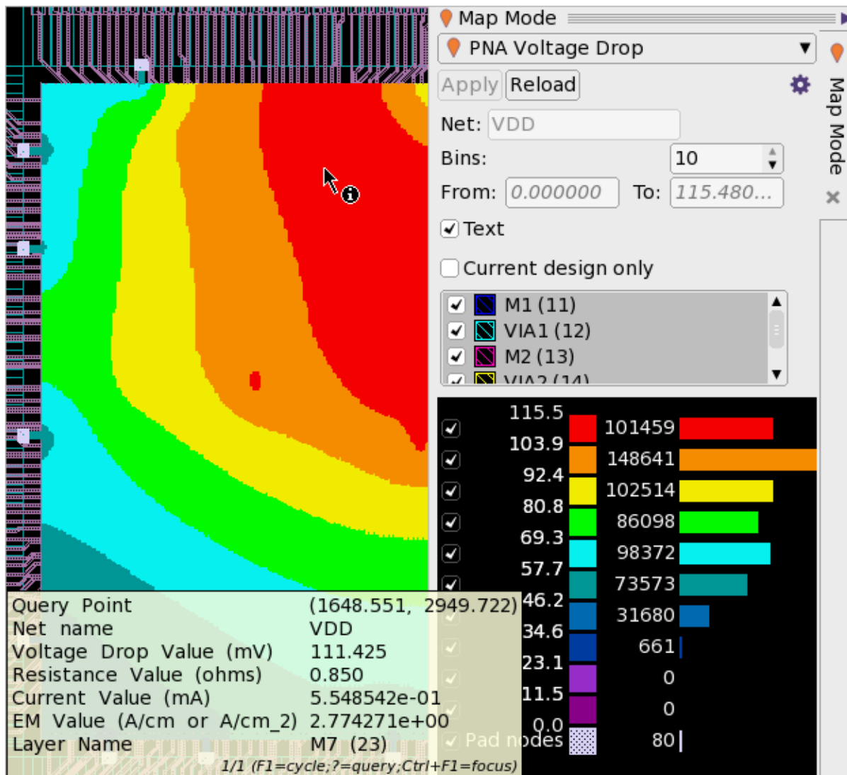
Figure 117 PNA Voltage Drop
