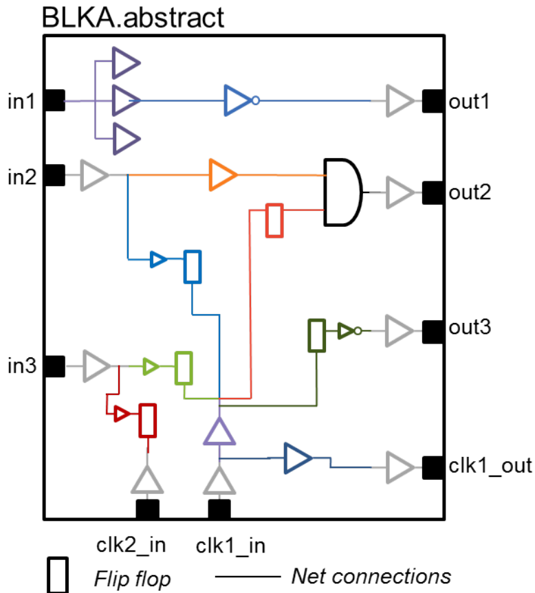
Figure 26 Example Black Box Timing Model
