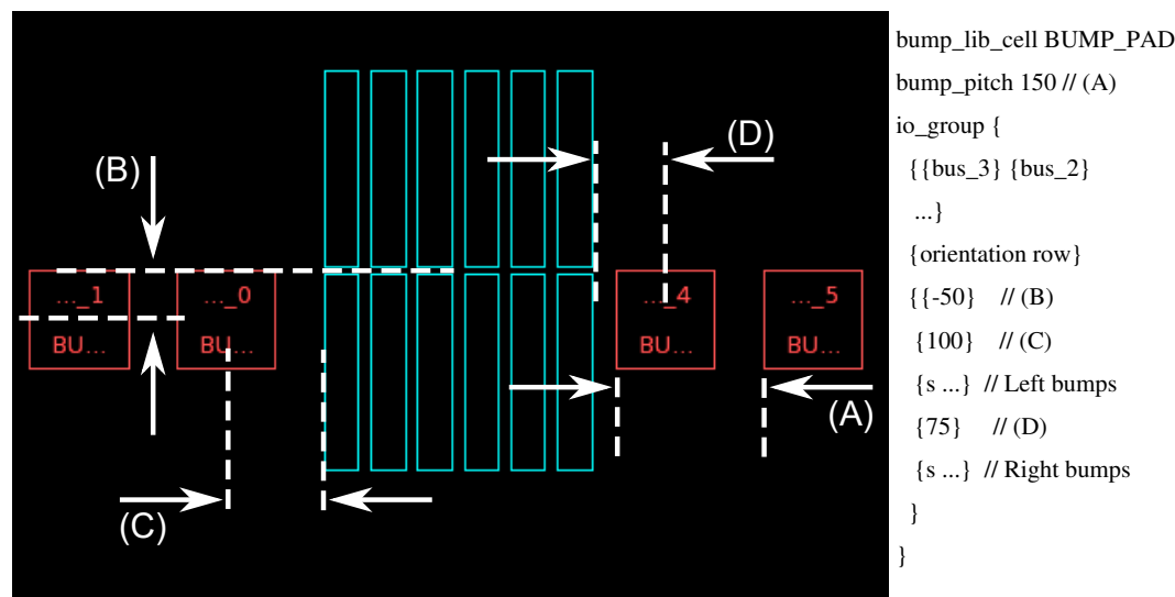
Figure 32 Bump Cell Offsets and Spacings
