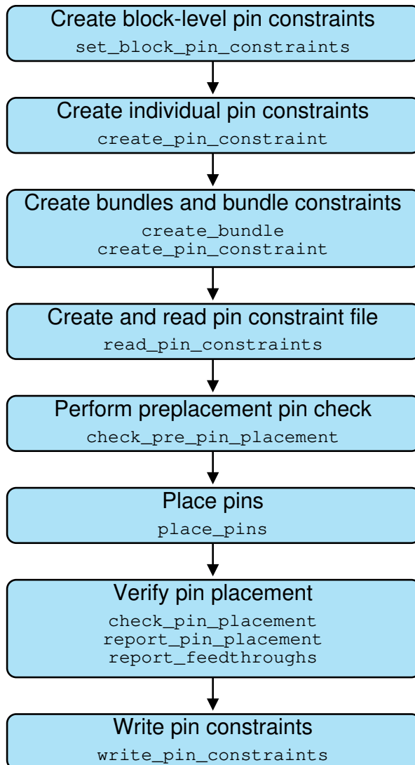
Figure 145 Pin Assignment Flow
