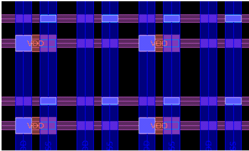
Figure 99 Composite Bridging Patterns
