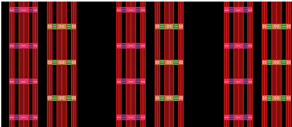
Figure 97 Bridging Straps
