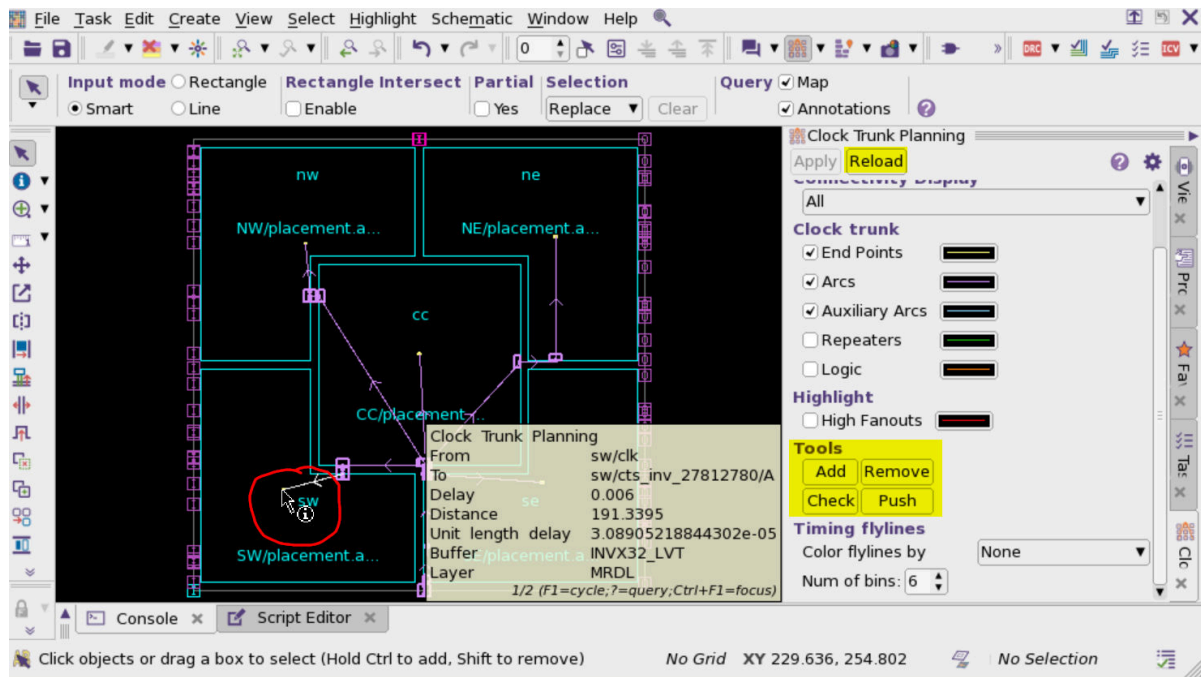
Figure 144 Clock Trunk Planning Panel
