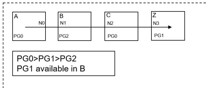
Figure 64 Feedthrough With Related Supply on Feedthrough Ports
