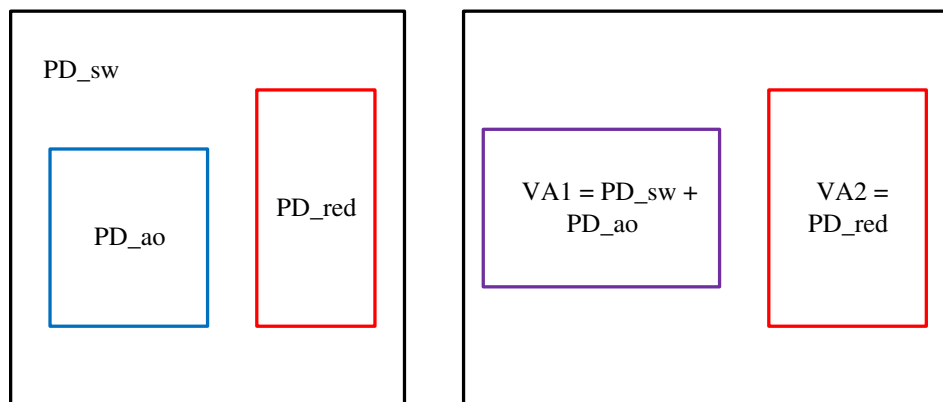
Figure 65 Merging Power Domains to a Common Voltage Area
