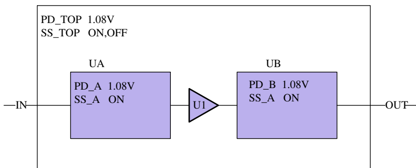
Figure 60 Always-On Buffer Using a Bias Supply
