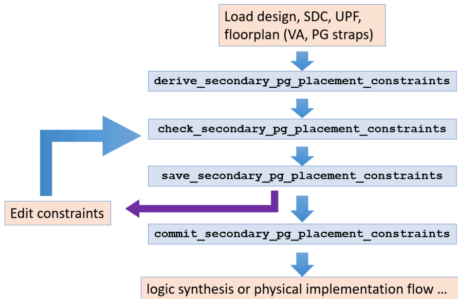
Figure 68 Interactive Flow for Secondary PG Constraint Creation
