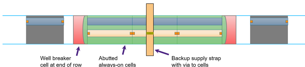
Figure 70 Always-On Cells in the Layout
