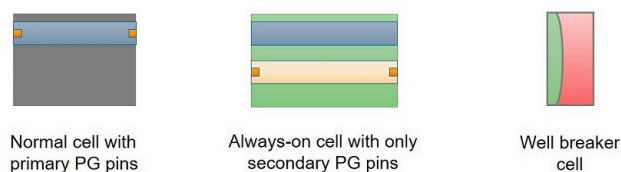
Figure 70 Always-On Cells in the Layout
