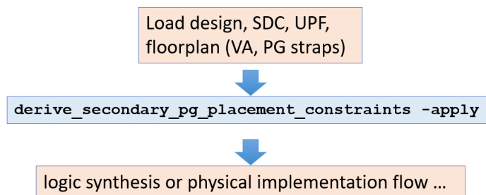
Figure 67 Automatic Creation of Secondary PG Constraints
