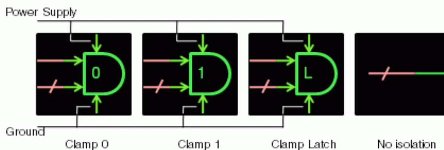
Figure 38 Representation of Various Types of Isolation Cells
