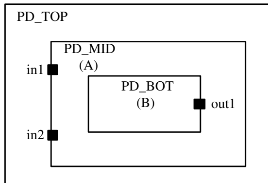
Figure 57 Isolation Cell Insertion With the Parent Location Specified
