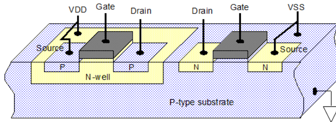
Figure 73 CMOS Technology Without Well Bias
