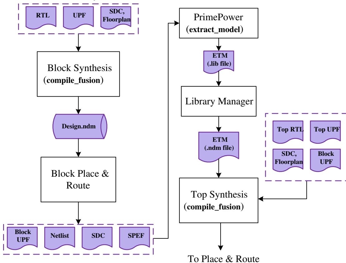
Figure 50 Hierarchical Synthesis Flow for ETMs and Macros
