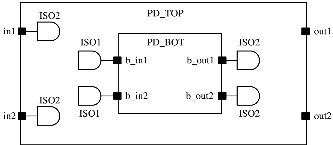
Figure 56 Isolation Cell Insertion With the Domain Boundary Specified
