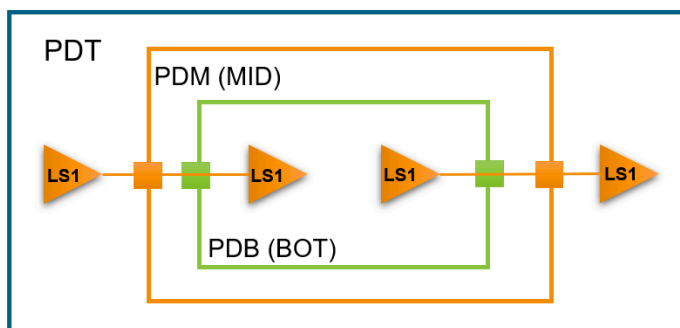
Figure 24 Nested Power Domains With Level Shifters
