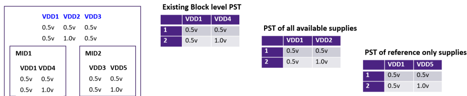
Figure 47 Derived block PSTs after design partition
