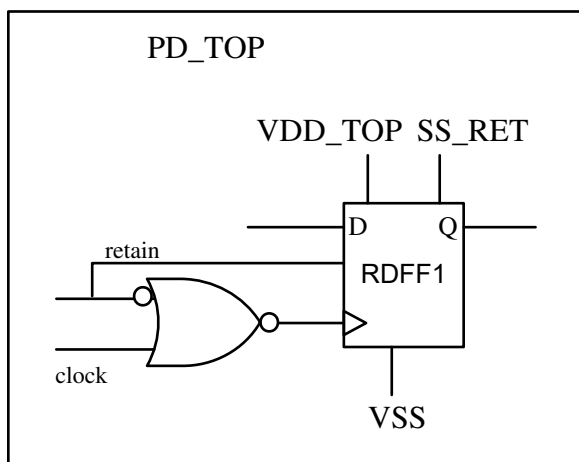
Figure 10 Zero-Pin Retention Register
