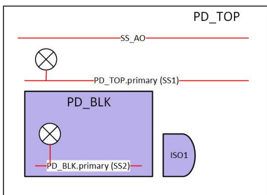
Figure 75 Bias Supplies and Isolation Cells
