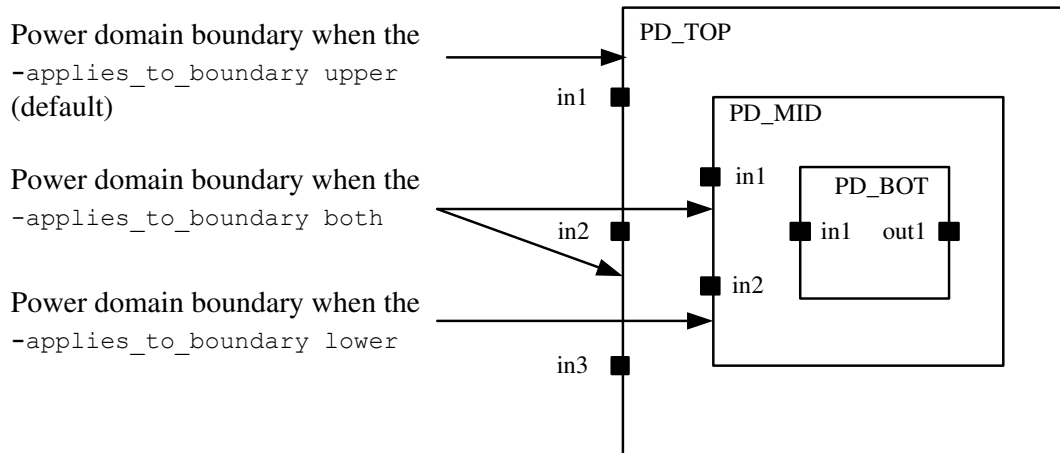
Figure 54 Definition of Power Domain Boundaries for PD_TOP
