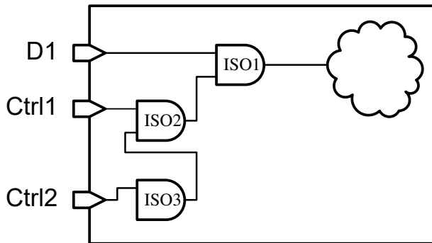
Figure 36 Third Step in Isolation Cell Insertion
