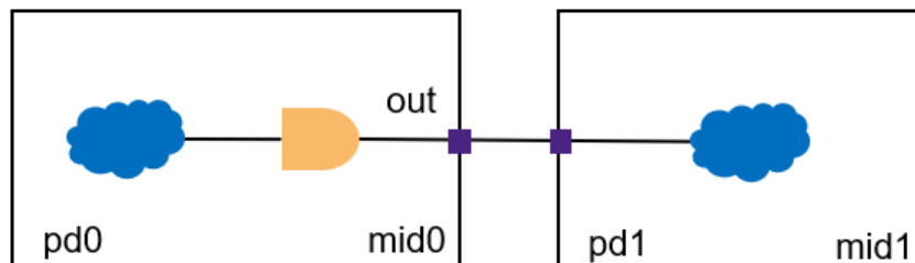
Figure 76 generate_upf_strategies Illustration
