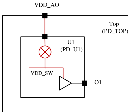
Figure 51 Example of an ETM in a Design
