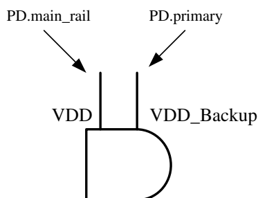
Figure 66 Supply Connections for Dual-Rail Cell
