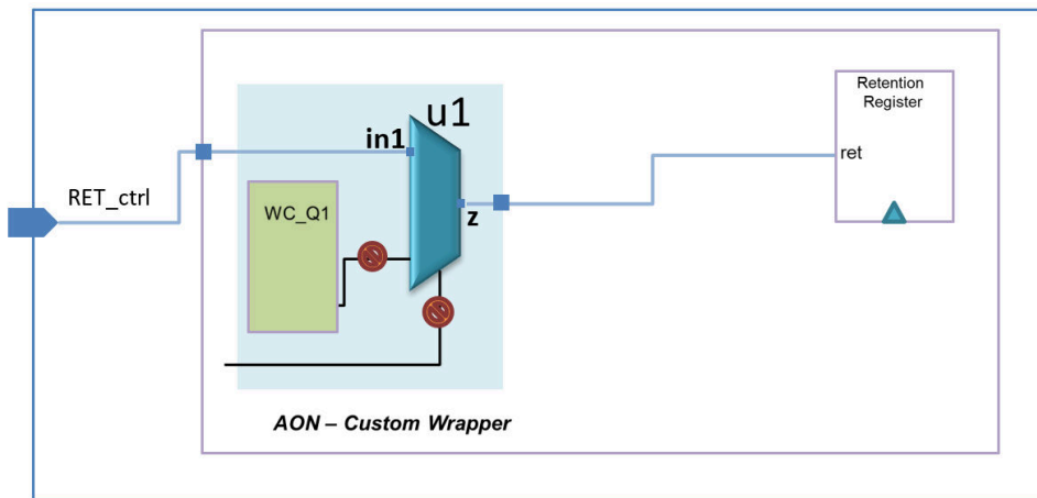
Figure 72 Example Wrapper Cell Wrapping RET_ctrl Control Signal, With Possible Isolation/LS Violations Marked
