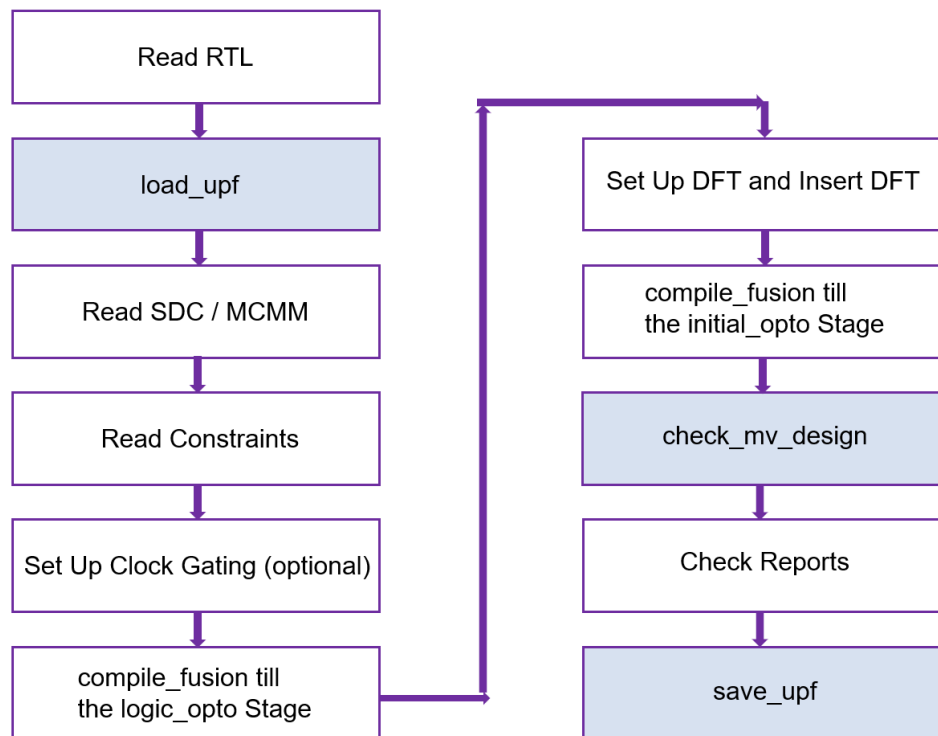
Figure 12 Synthesis Flow for Multivoltage Designs
