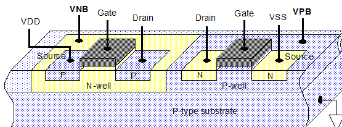
Figure 74 CMOS Technology With N-Well and P-Well Bias
