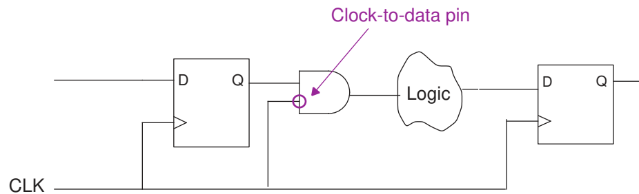
Figure 9 Clock-to-Data Pin
